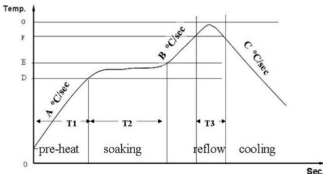
Figure 5: Reflow Profile for RAK11300
