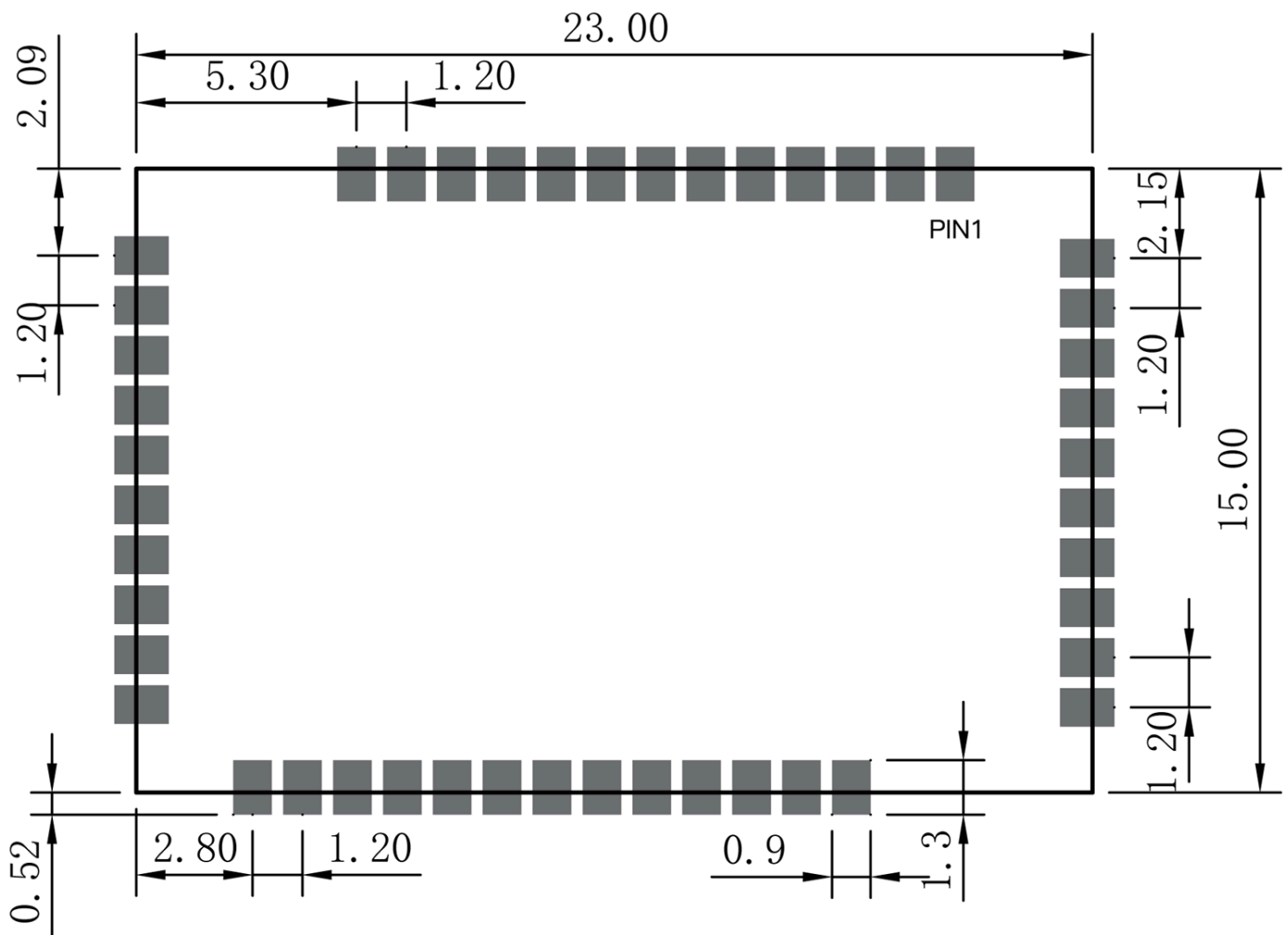
Figure 4: RAK11300 Layout
