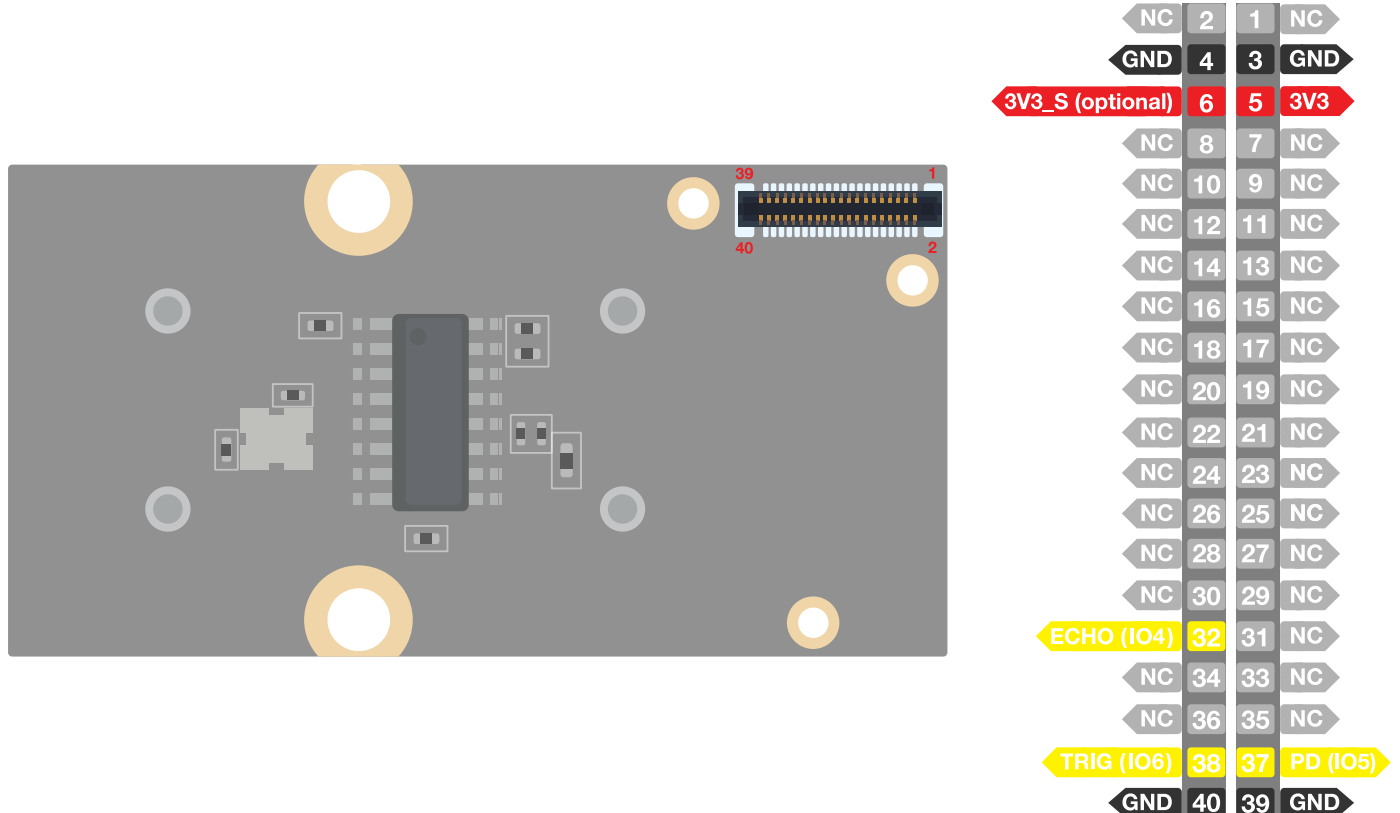
Figure 5: RAK12007 WisBlock Ultrasonic Sensor Module Pinout
