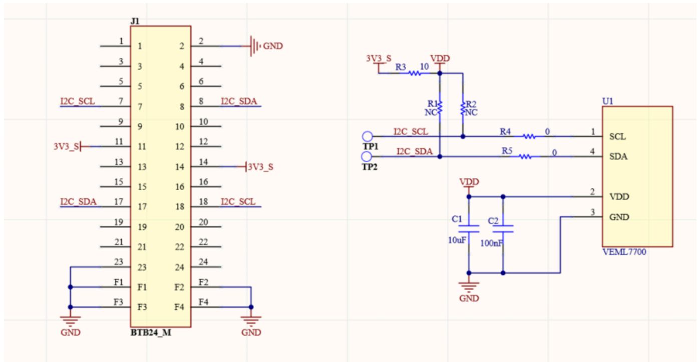
Figure 5: RAK12010 WisBlock Module Schematics
