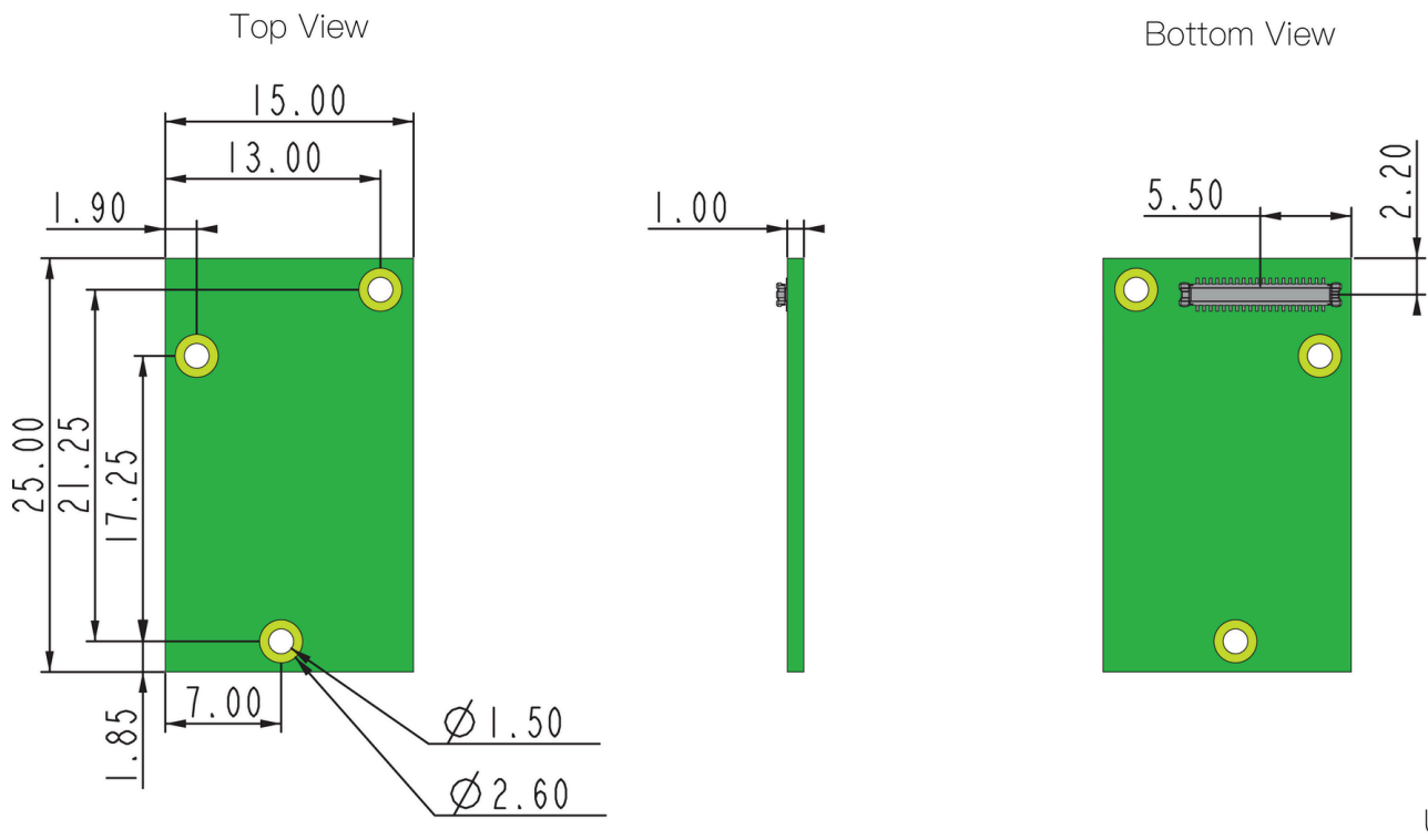
Figure 4: RAK12016 Mechanical Dimensions
