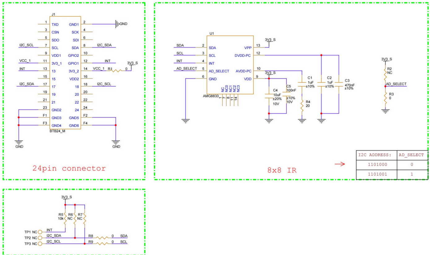
Figure 6: RAK12040 WisBlock 8x8 IR Sensor schematics
