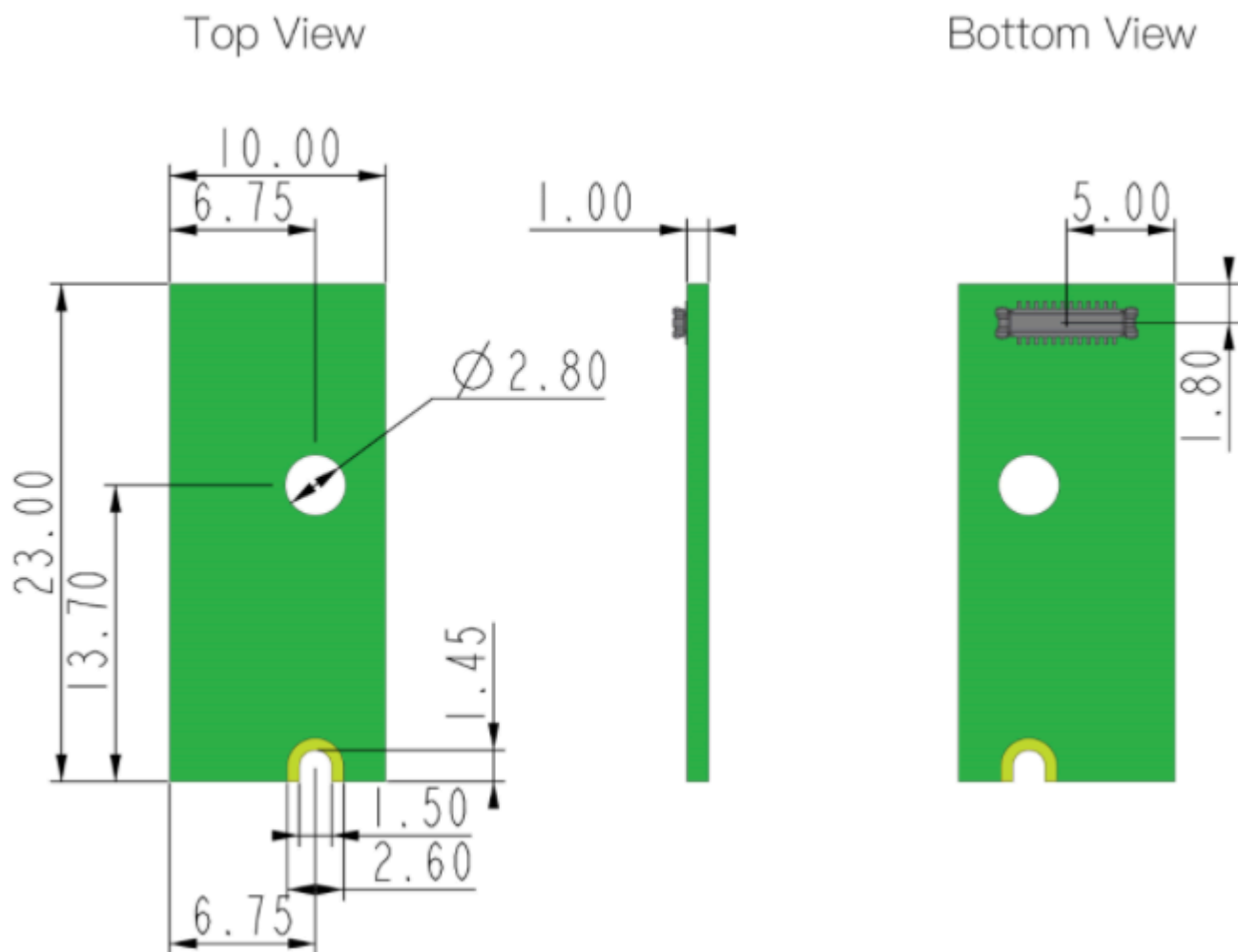
Figure 4: RAK12040 WisBlock 8x8 IR Sensor Mechanic Drawing
