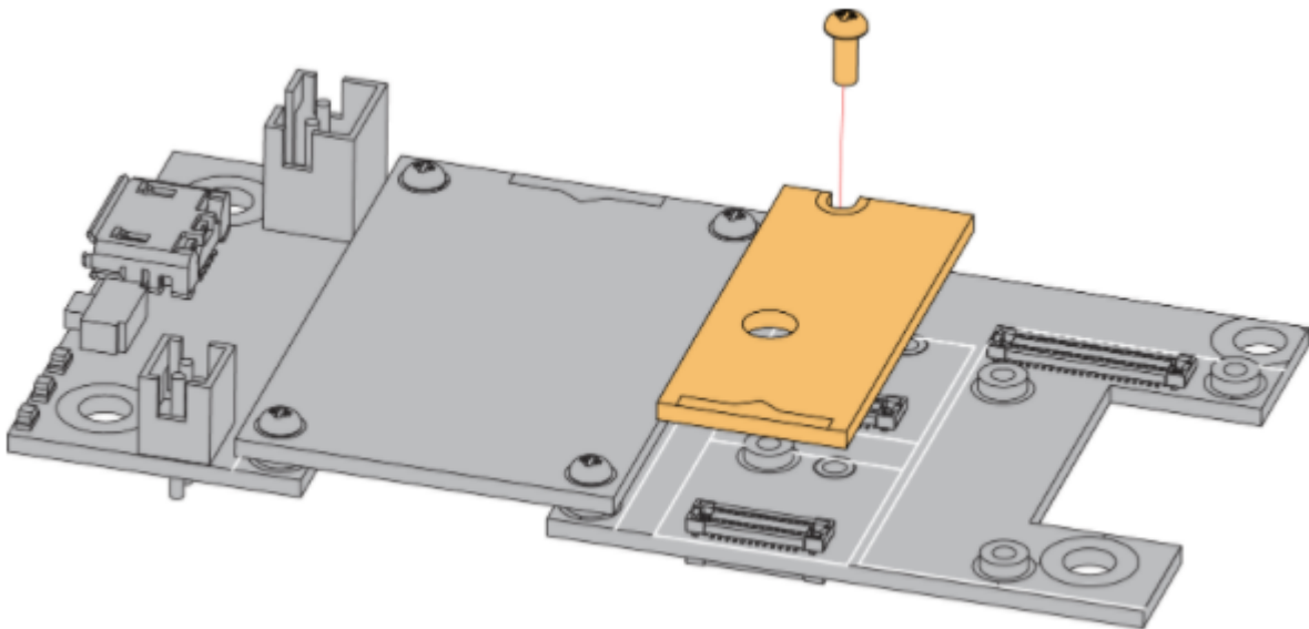
Figure 2: RAK12040 WisBlock 8×8 IR Sensor Mounting
