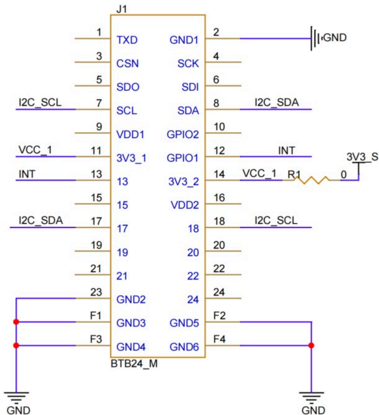
Figure 3: RAK12040 WisBlock 8x8 IR Sensor Pinout Diagram
