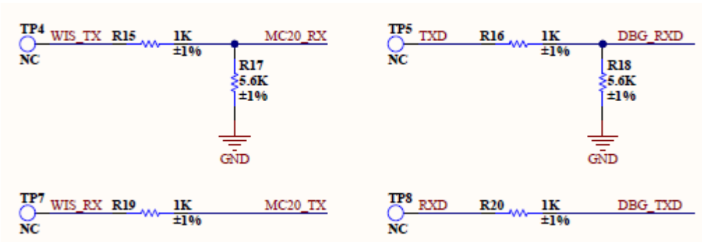
Figure 7: RAK13101 Voltage Level Shifter Circuit
