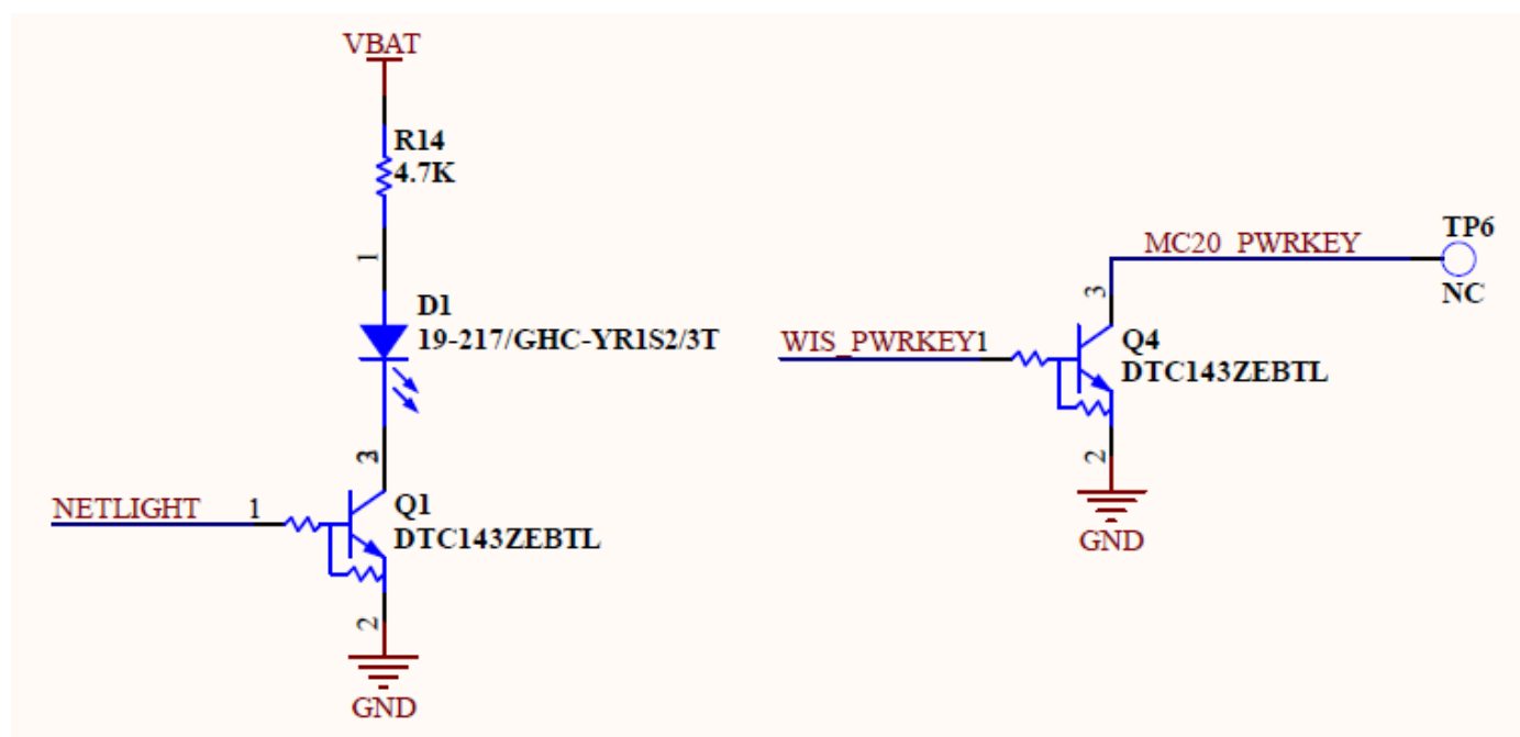
Figure 11: RAK13101 Module LED PWRKEY Control Circuit
