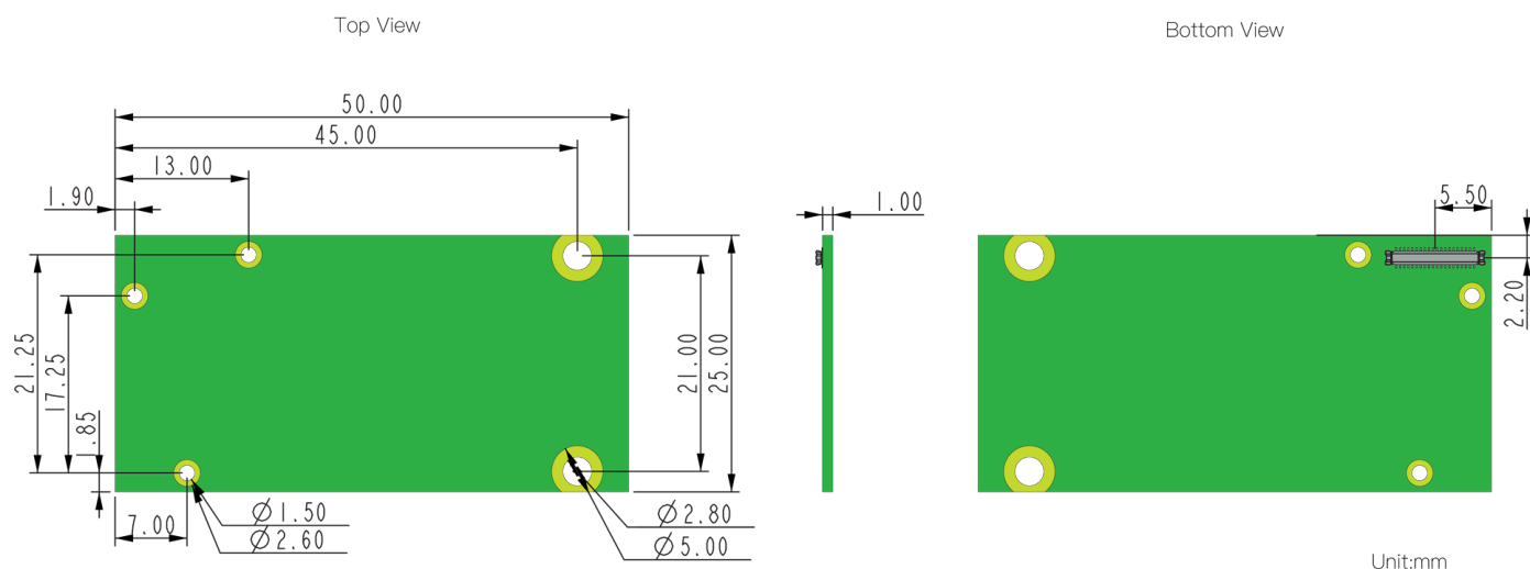
Figure 5: RAK13800 mechanical dimensions
