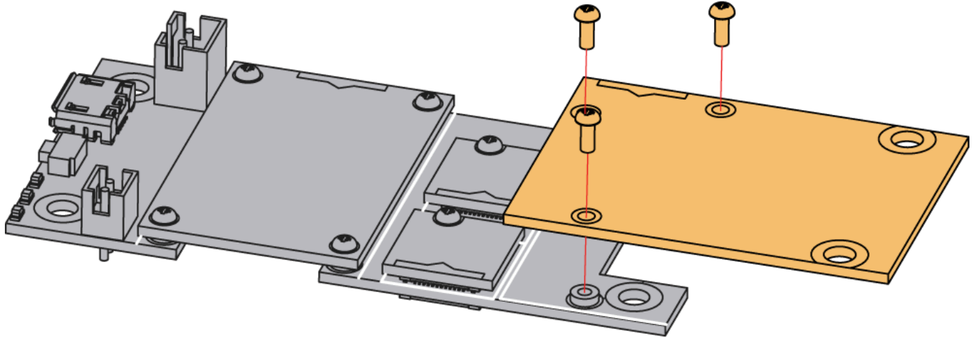
Figure 1: RAK13801 WisBlock Sensor mounting
