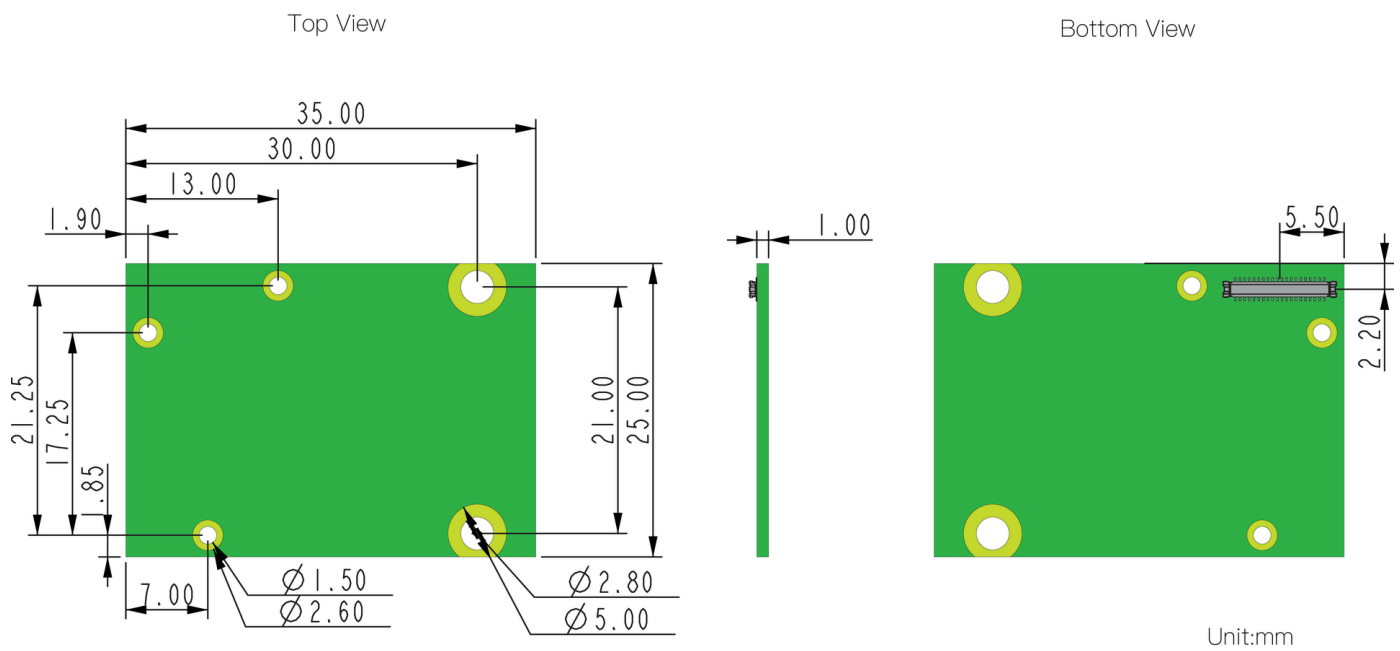
Figure 3: RAK13801 WisBlock Sensor mechanical drawing
