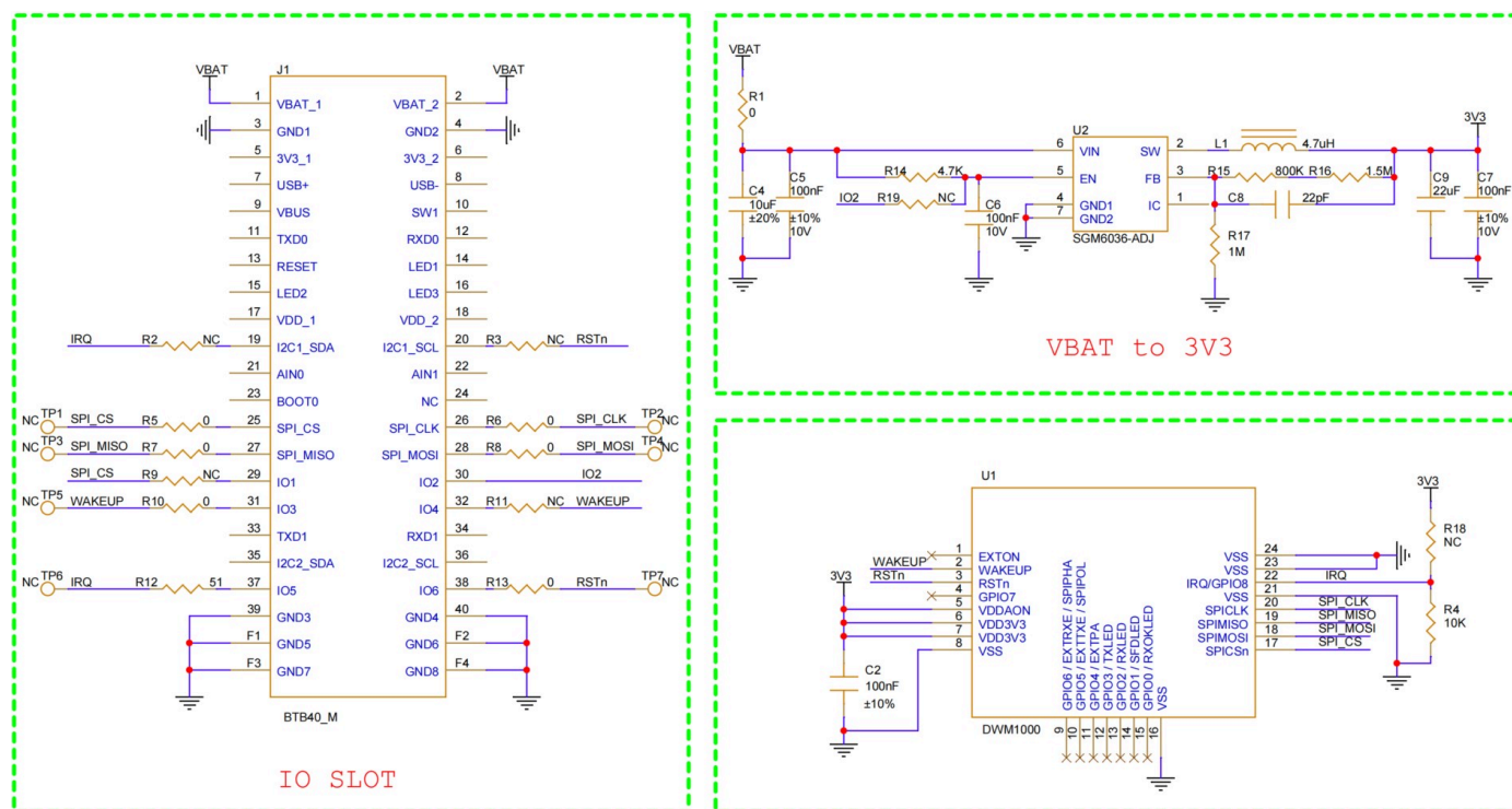
Figure 5: RAK13801 WisBlock Module schematics
