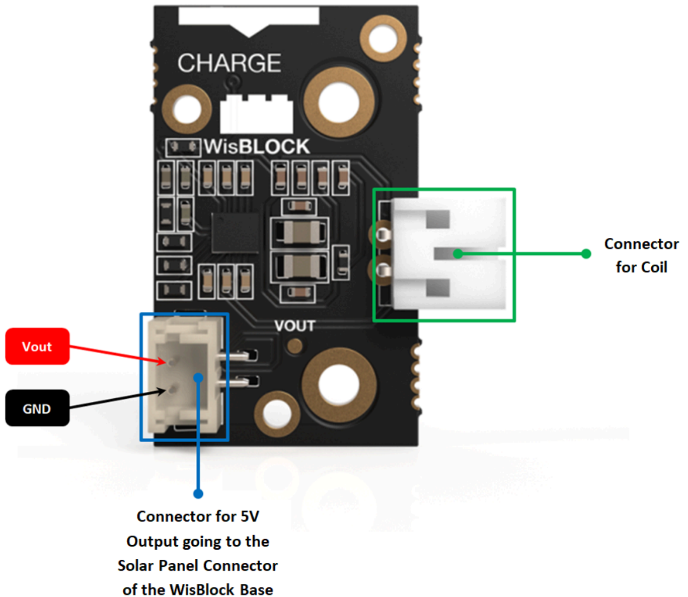
Figure 3: RAK19006 Pinout and Connector assignments
