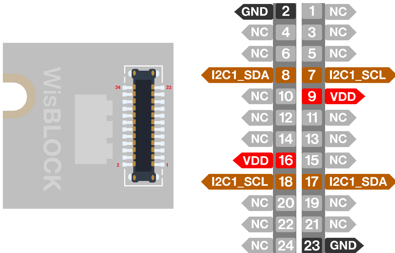
Figure 3: RAK1901 WisBlock Sensor Pinout Diagram
