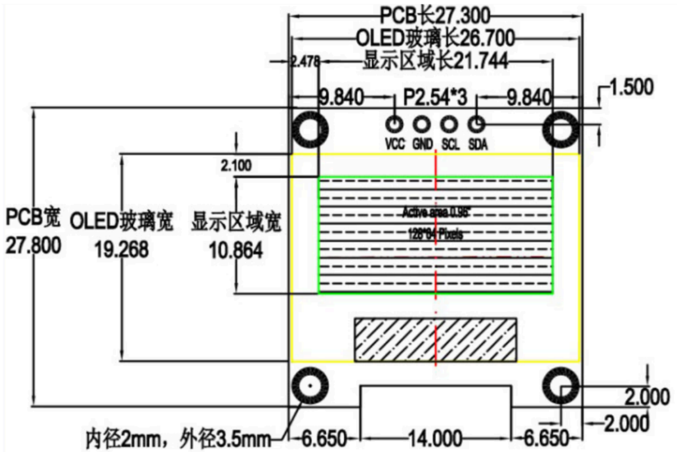
Figure 3: Mechanical Dimensions
