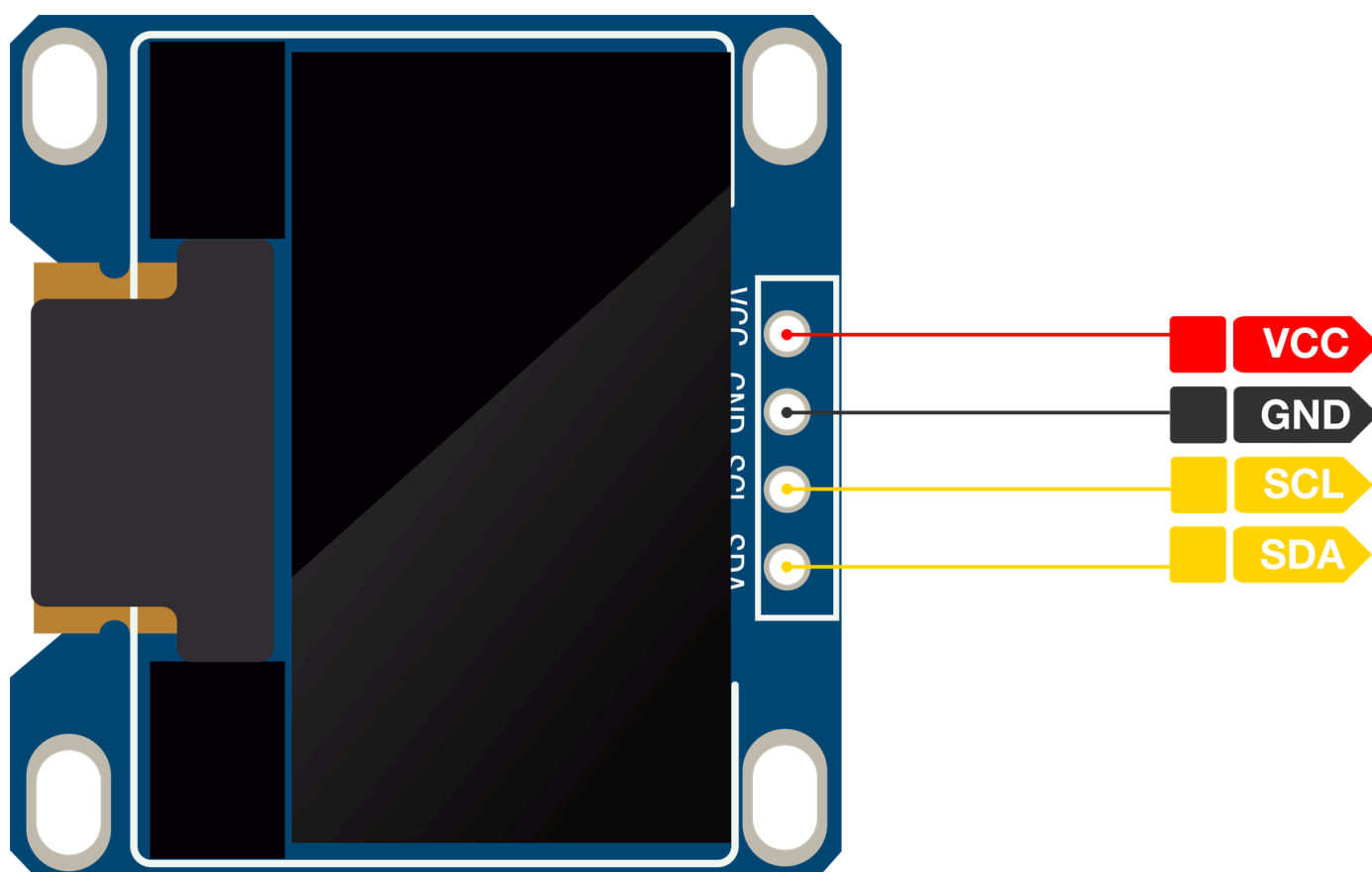
Figure 2: RAK1921 Pin Definition
