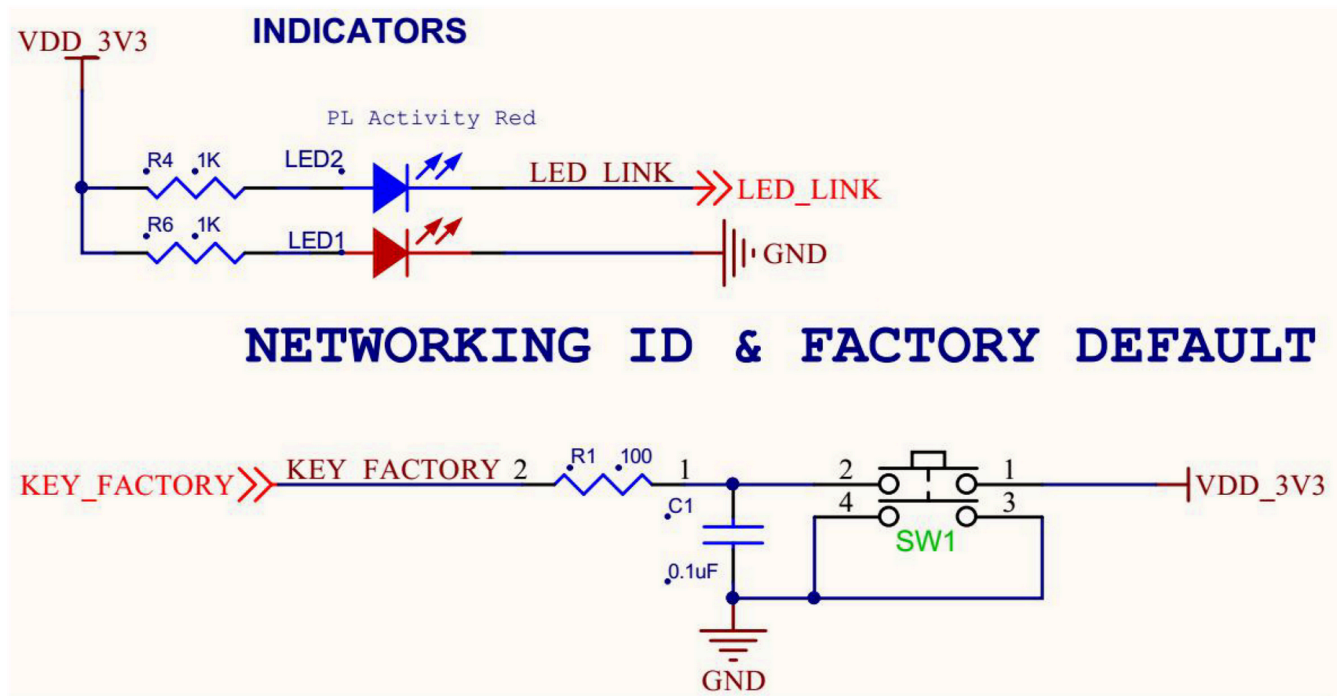
Figure 6: LED diagram
