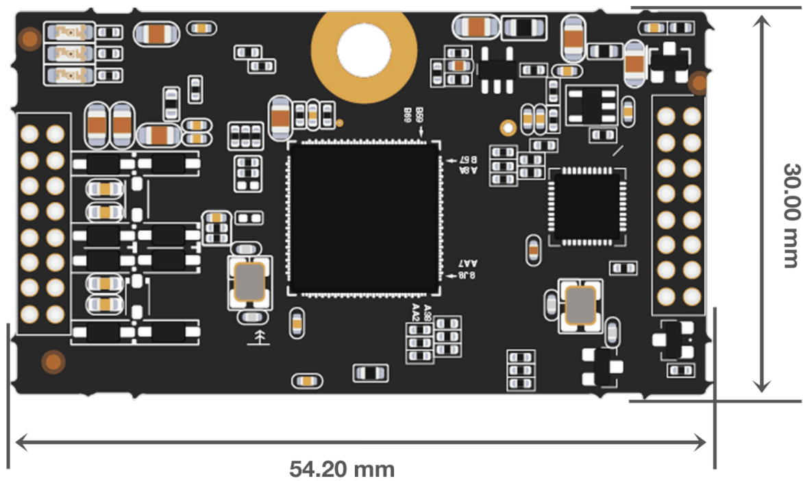
Figure 5: Module dimensions
