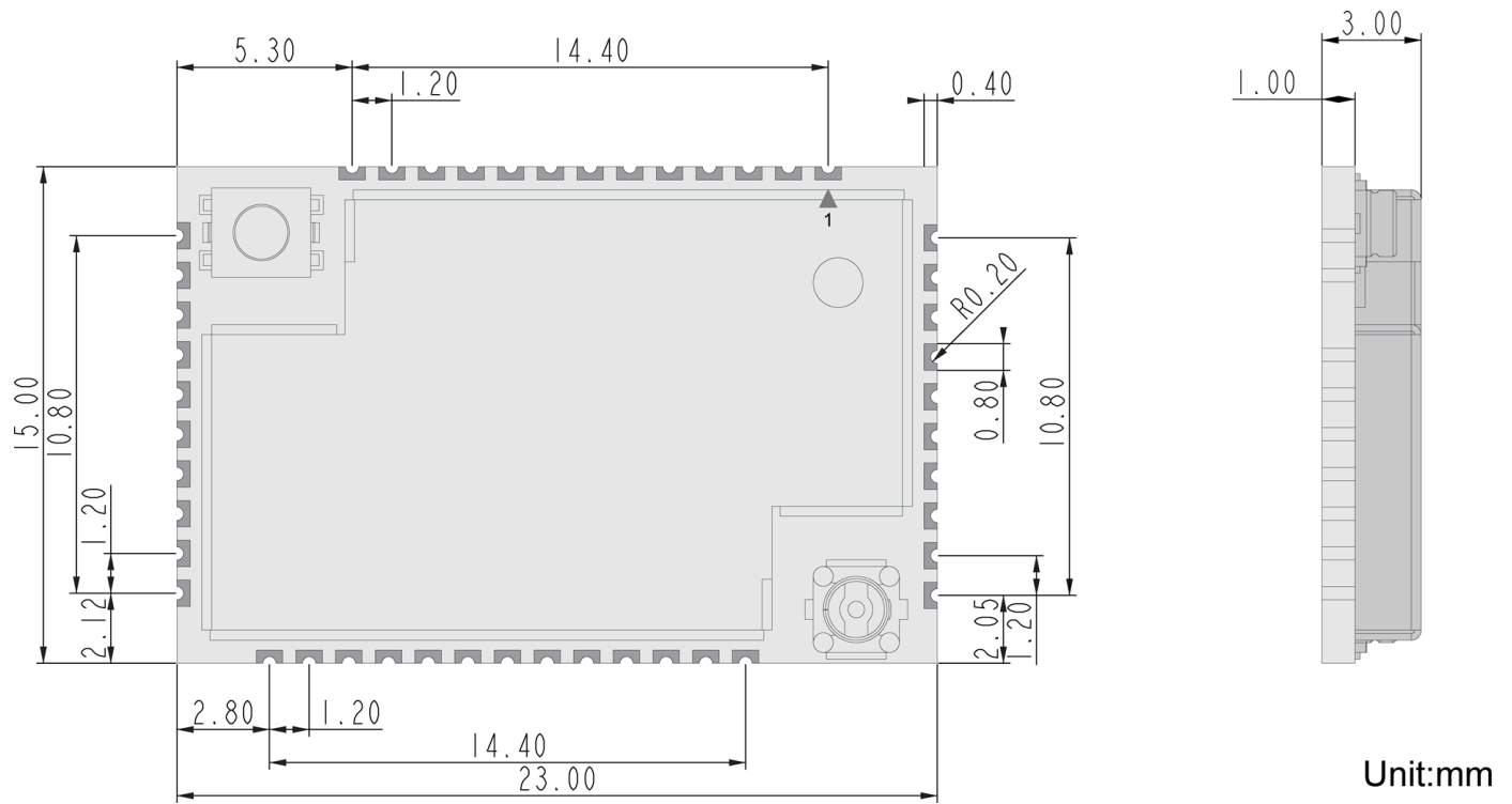
Figure 3: RAK11300 Physical Dimension
