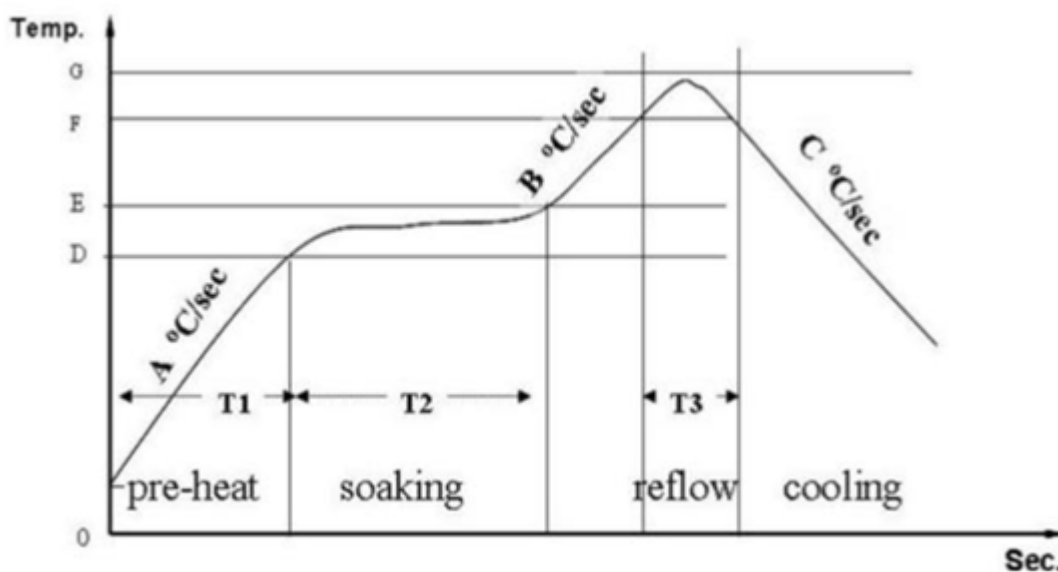
Figure 5: Reflow Profile for RAK11300
