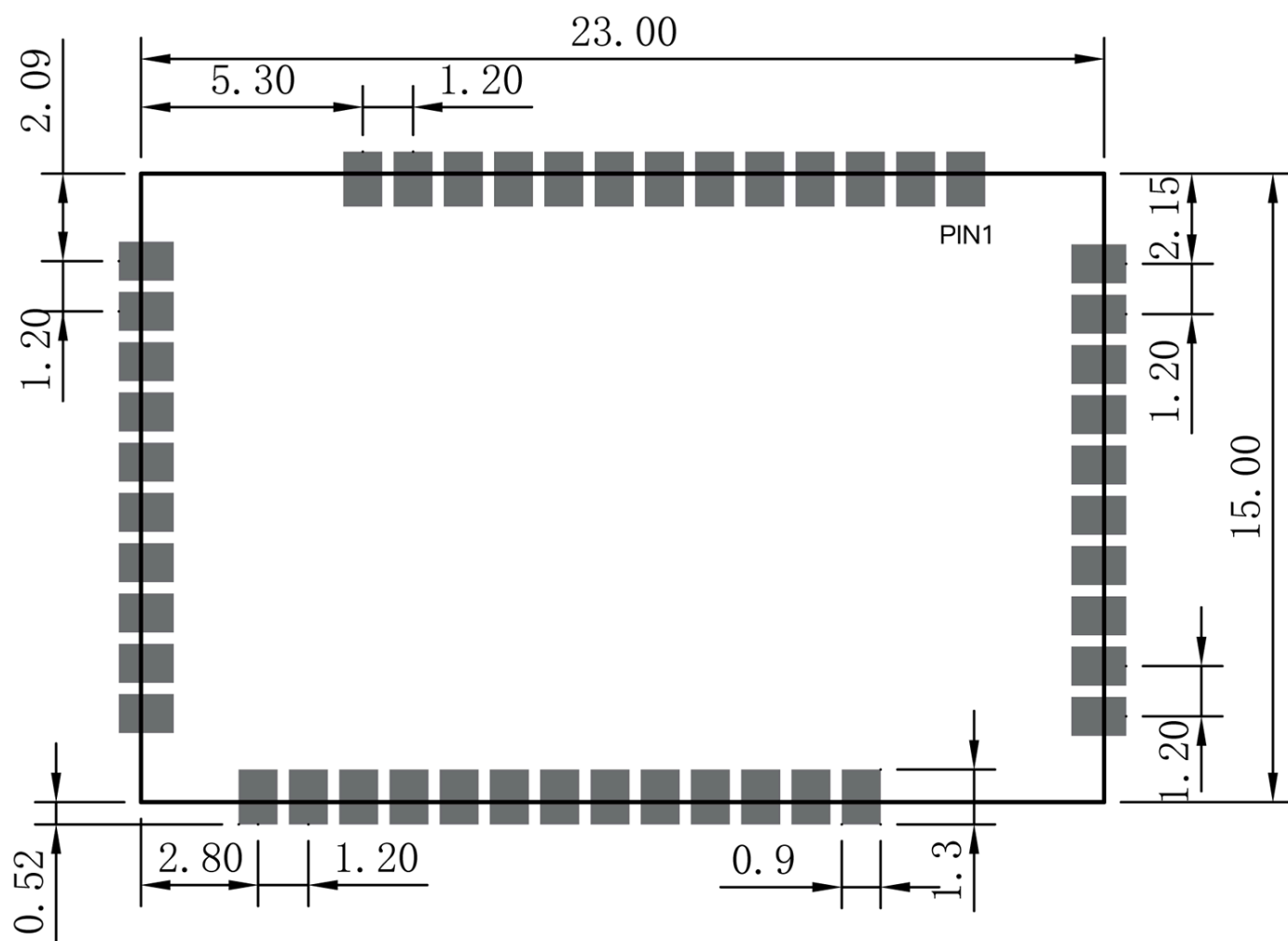
Figure 4: RAK11300 Layout
