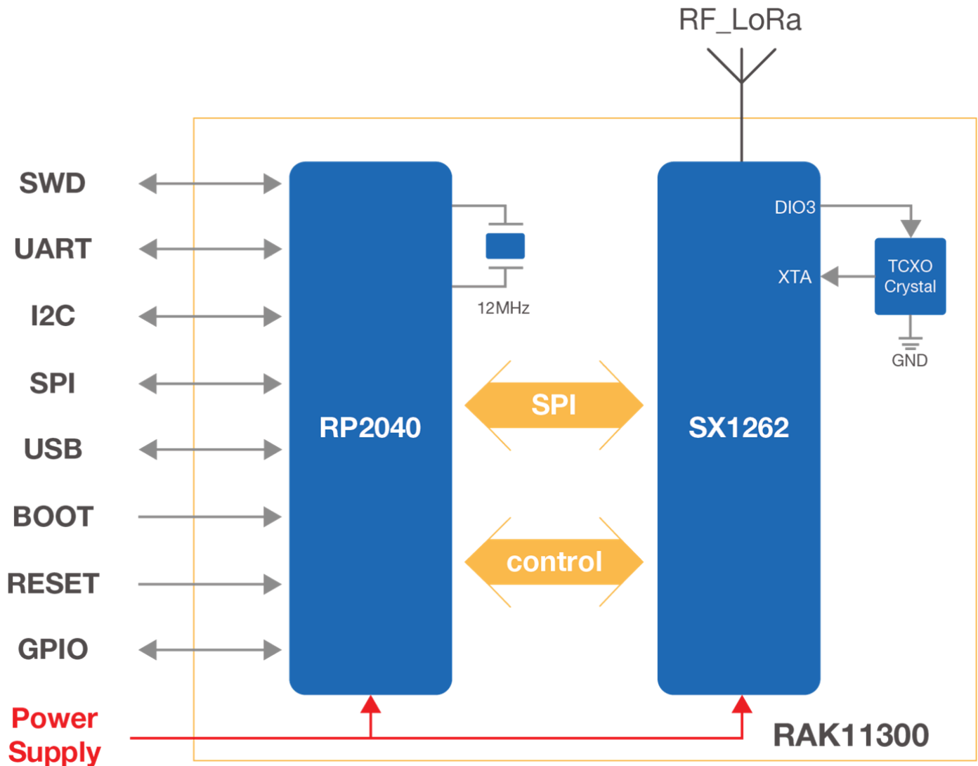
Figure 1: RAK11300 System Block Diagram
