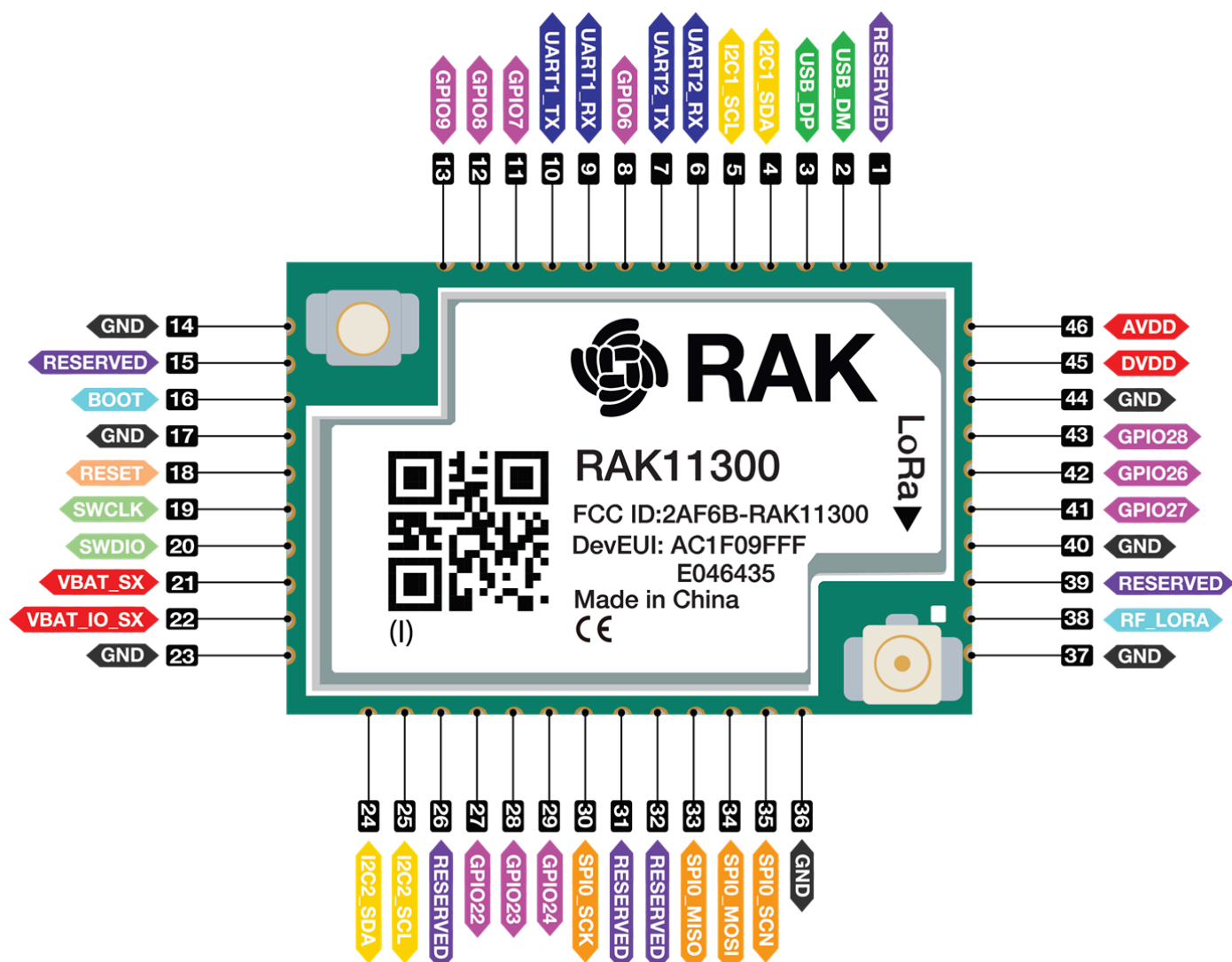
Figure 2: RAK11300 Module Pinout
