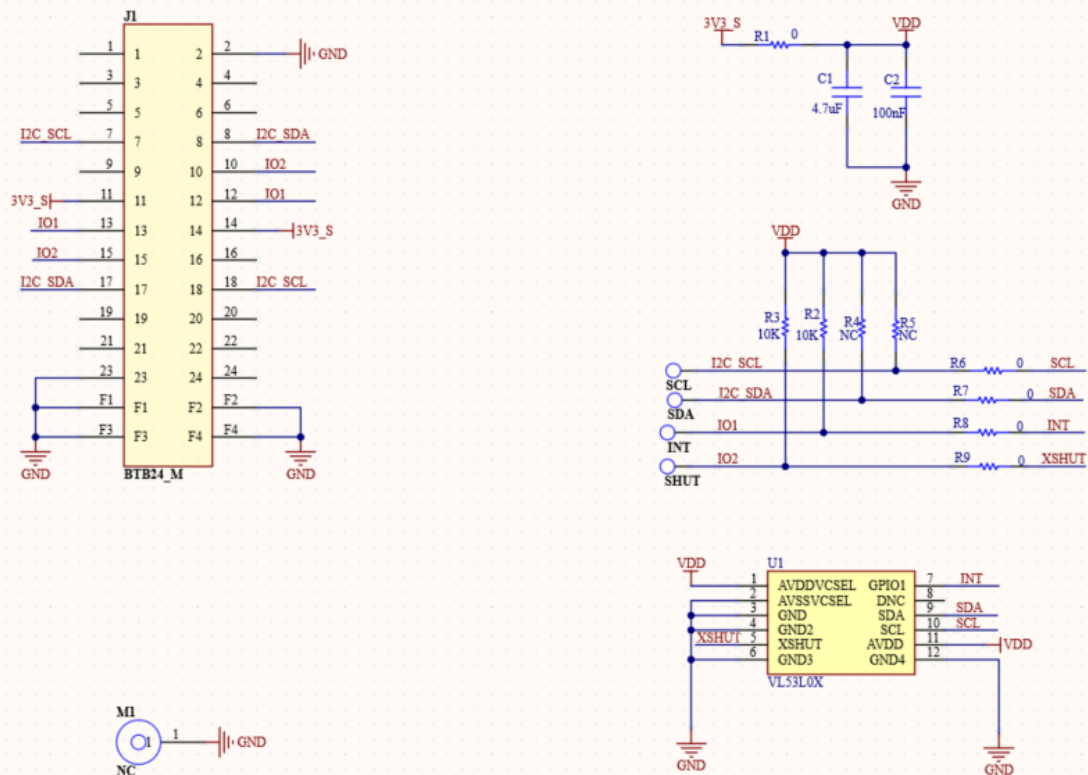
Figure 5: RAK12014 WisBlock ToF Module Schematic
