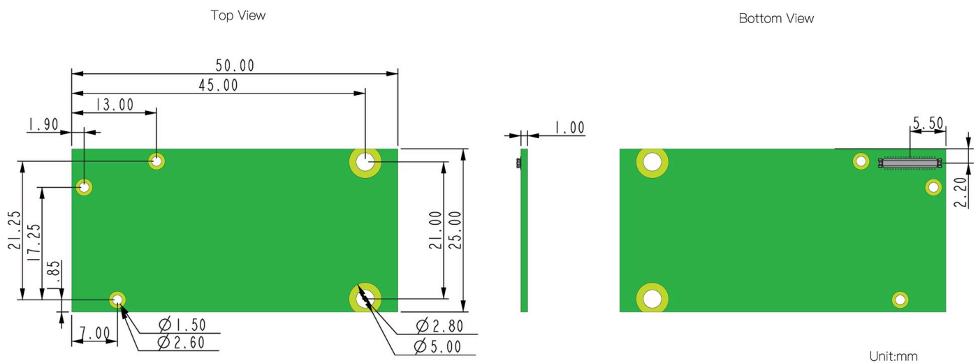
Figure 4: RAK12037 WisBlock Sensor mechanical drawing
