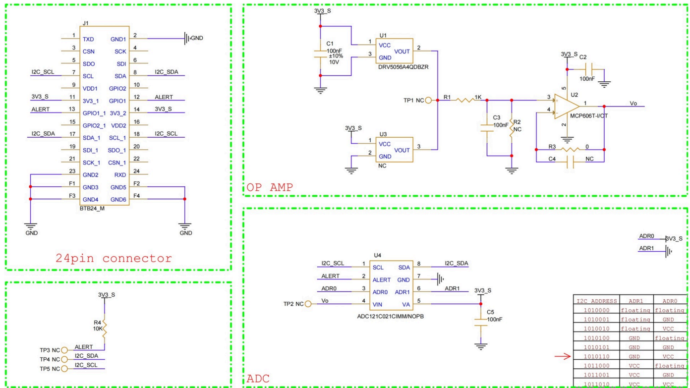
Figure 6: RAK12044 WisBlock Hall Effect Sensor schematics
