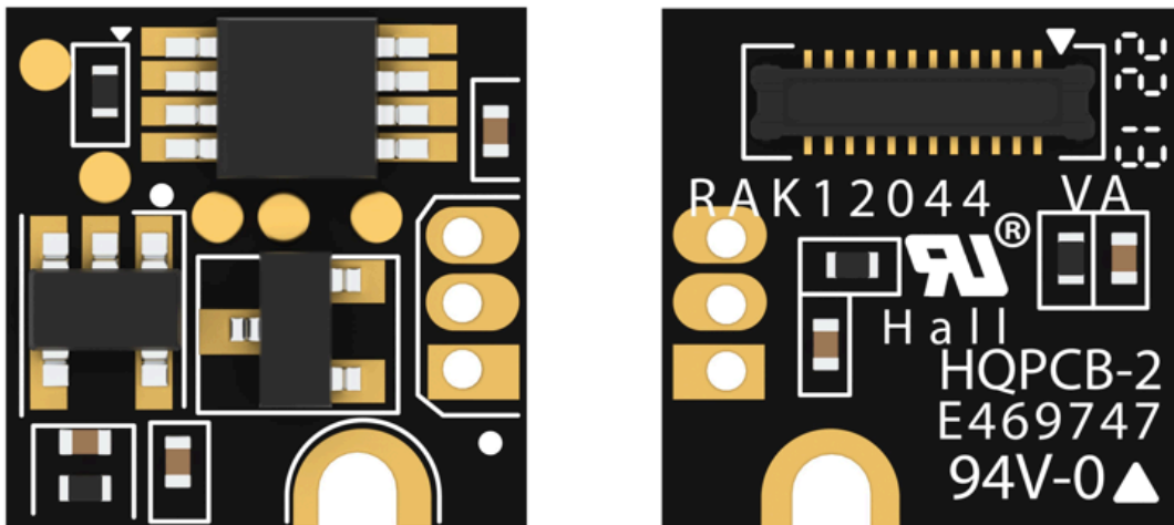
Figure 1: RAK12044 WisBlock Hall Effect Sensor
