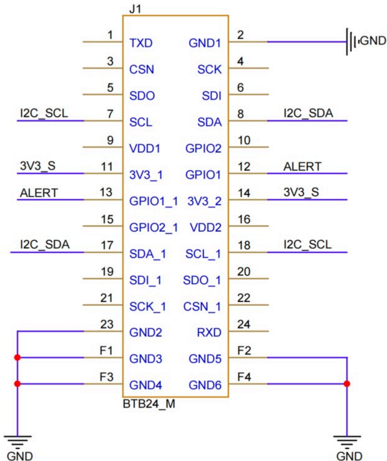
Figure 3: RAK12044 WisBlock Hall Effect Sensor Pinout Diagram
