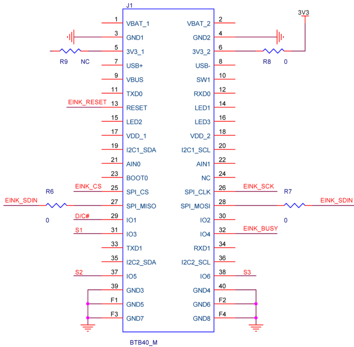
Figure 4: RAK14000 40-pin WisConnector Connection Schematic
