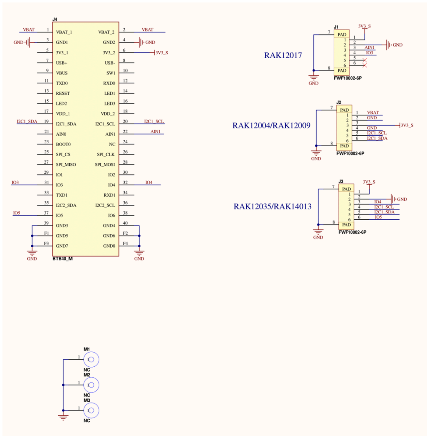
Figure 6: RAK14007 WisBlock Interface Module schematics
