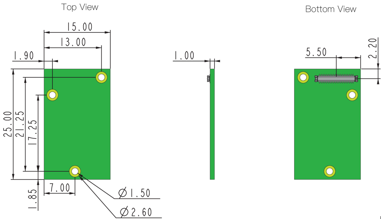
Figure 4: RAK14007 mechanical dimensions
