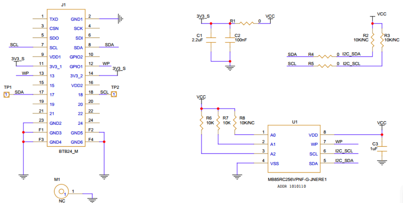
Figure 6: RAK15003 WisBlock 32kByte FRAM Module schematics
