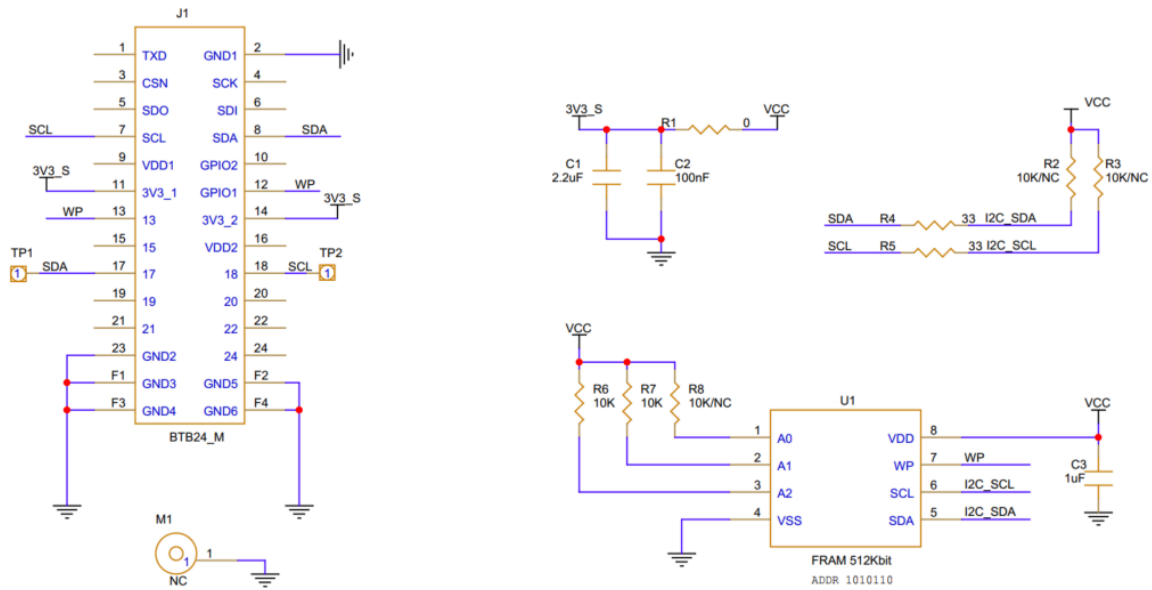
Figure 7: RAK15004 schematic diagram
