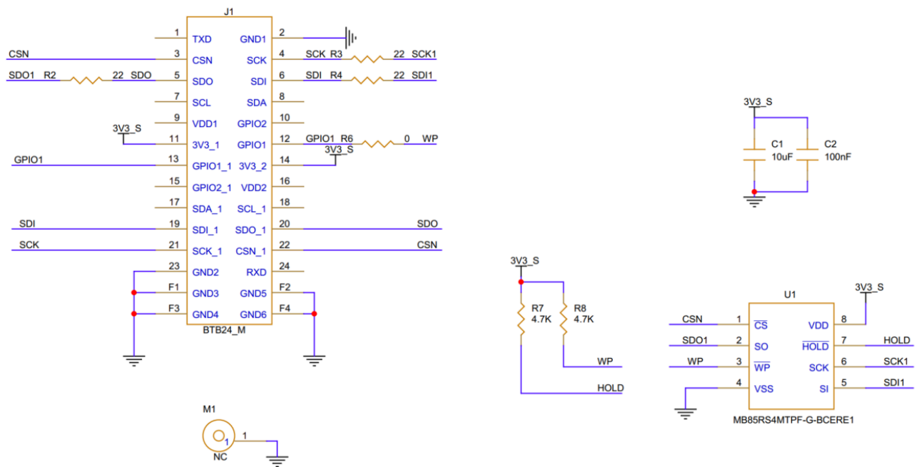
Figure 6: RAK15006 WisBlock FRAM Module schematics
