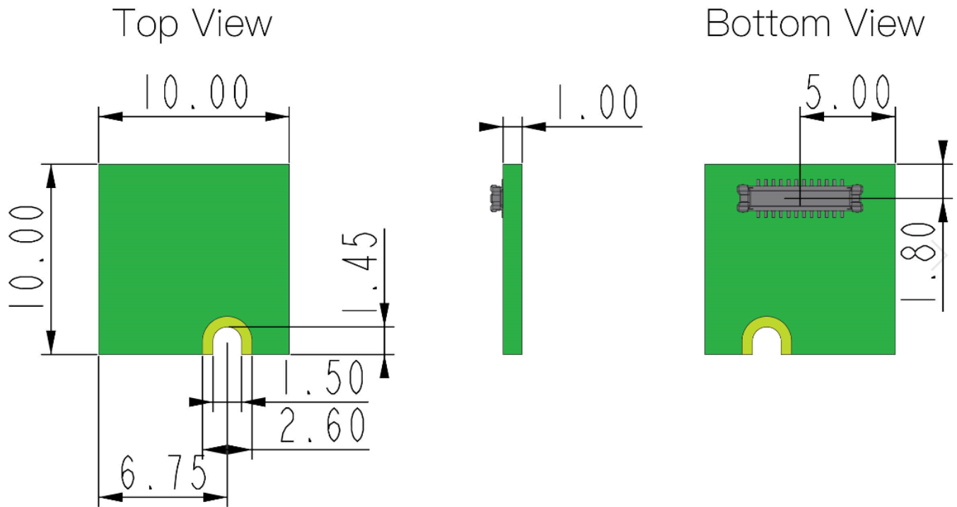
Figure 4: RAK15006 WisBlock FRAM Module Mechanic Drawing
