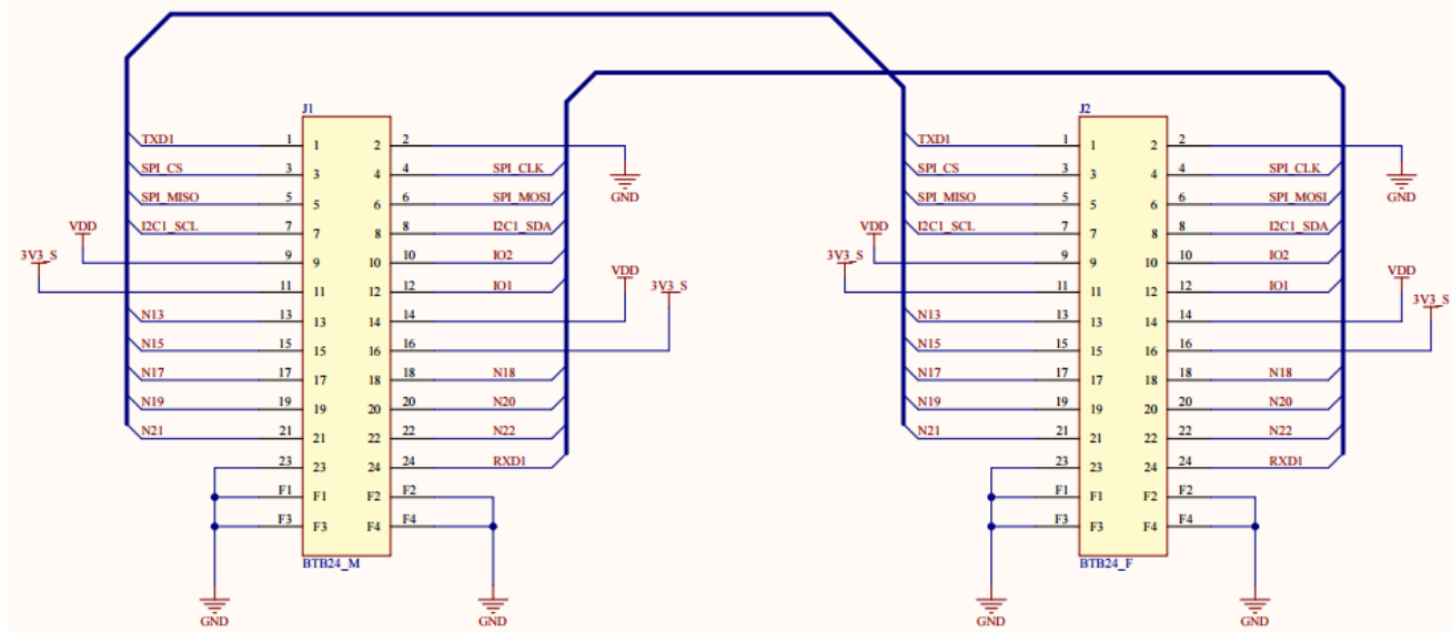
Figure 2: RAK19005 WisBlock Sensor Extension Cable Schematic
