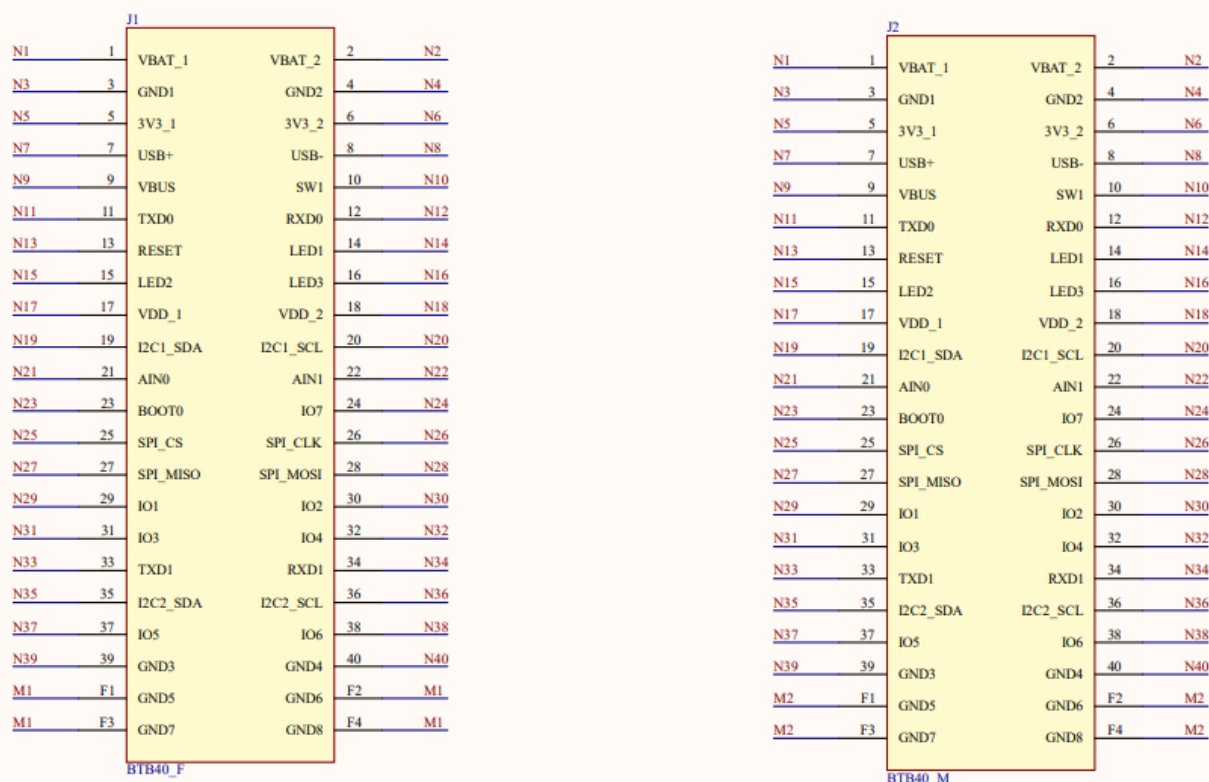
Figure 3: RAK19008 WisBlock IO Sensor Extension Cable Schematic
