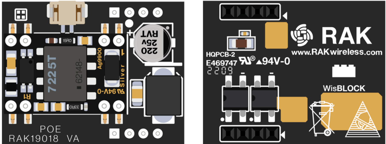
Figure 1: RAK19018 WisBlock PoE Module top (left) and bottom (right) view
