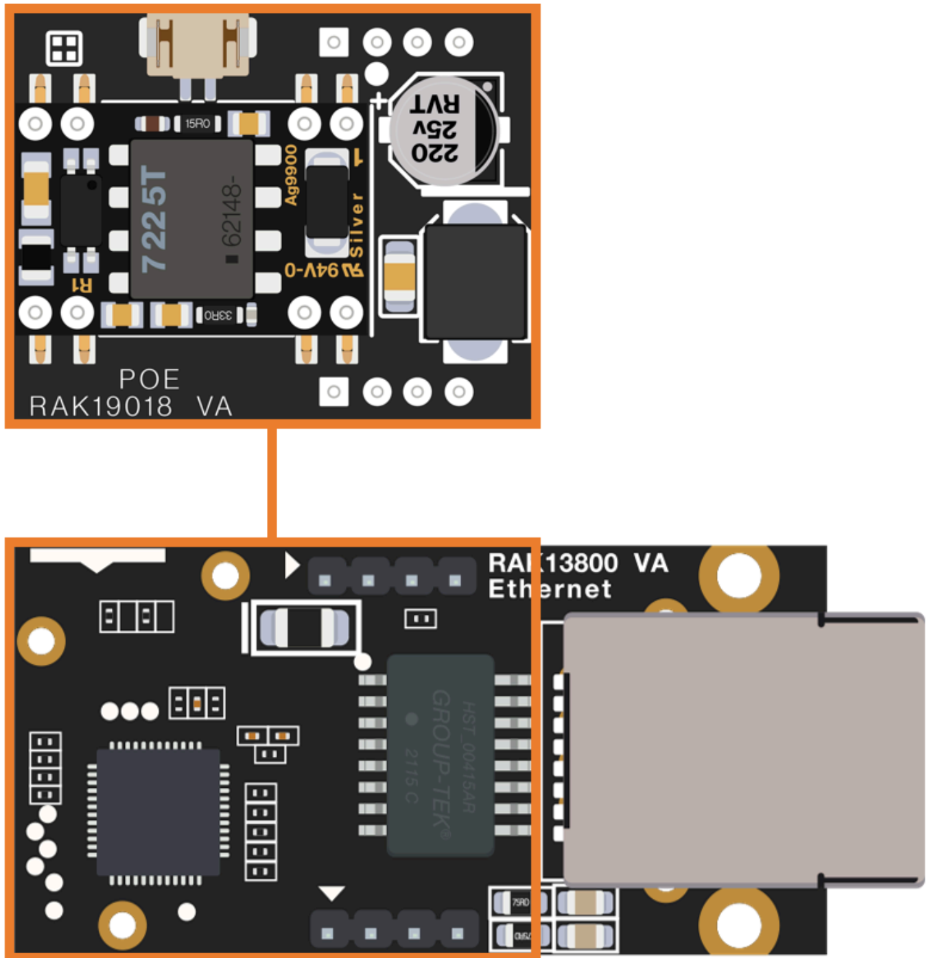
Figure 3: RAK19018 connection to RAK13800
