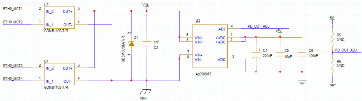
Figure 6: PoE Module
