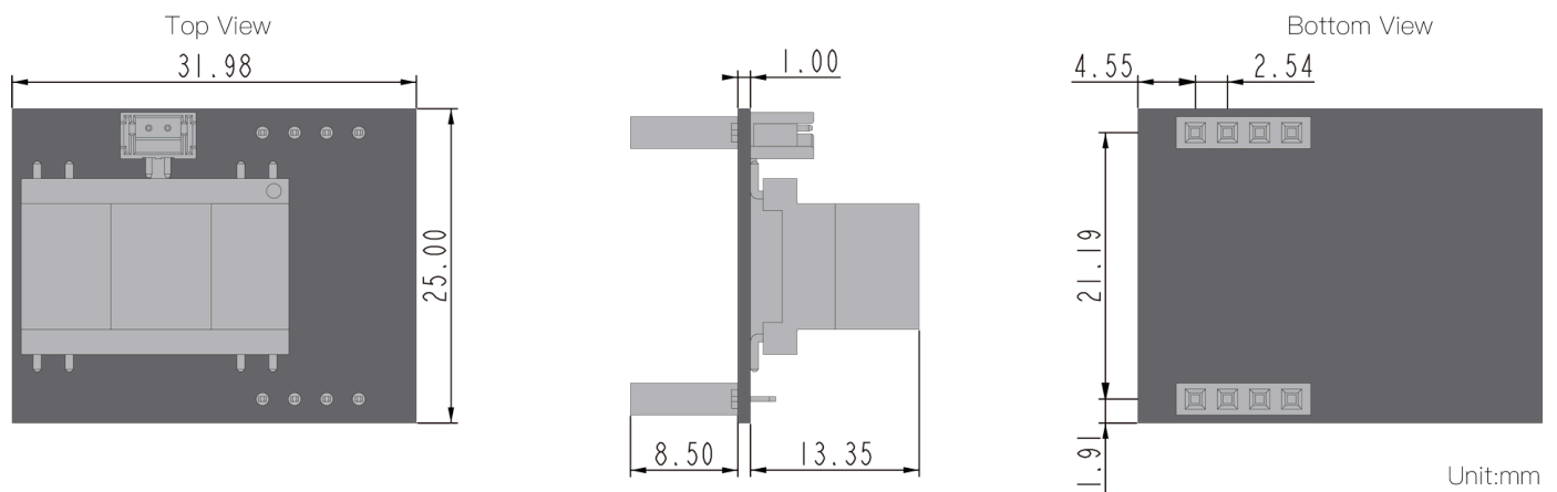
Figure 5: RAK19018 Mechanical Dimensions
