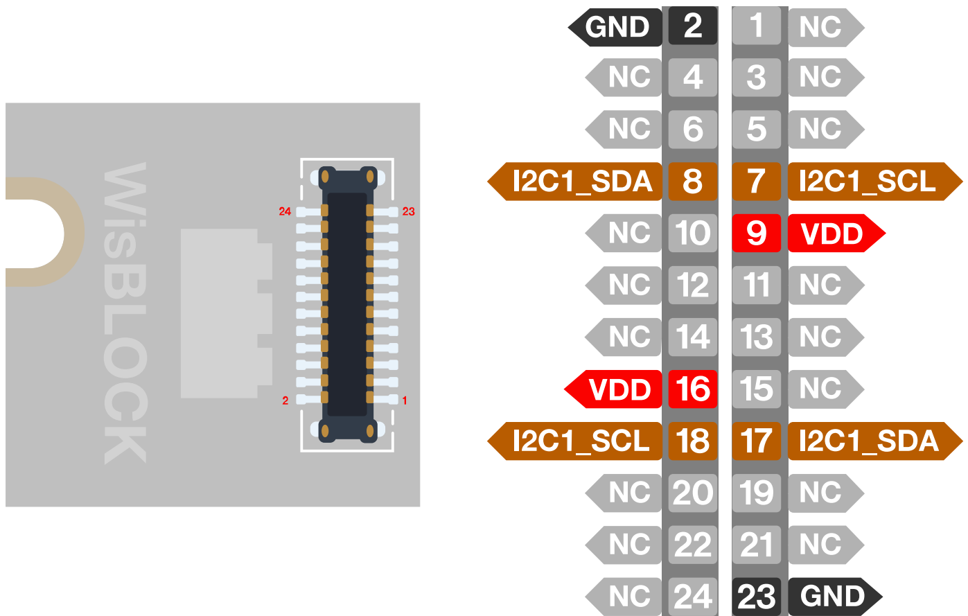
Figure 3: RAK1901 WisBlock Sensor Pinout Diagram
