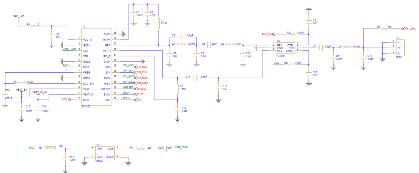
Figure 2: SX1262 Section
