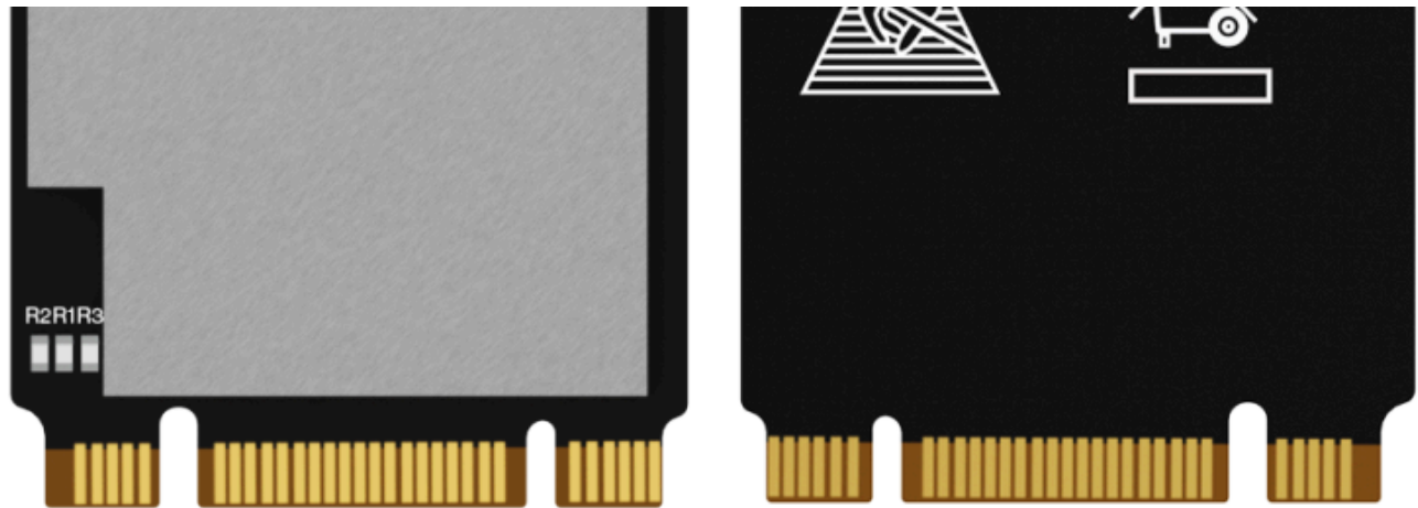
Figure 1: RAK5167 Board Overview
