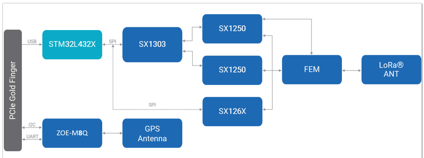
Figure 2: RAK5167 Block Diagram
