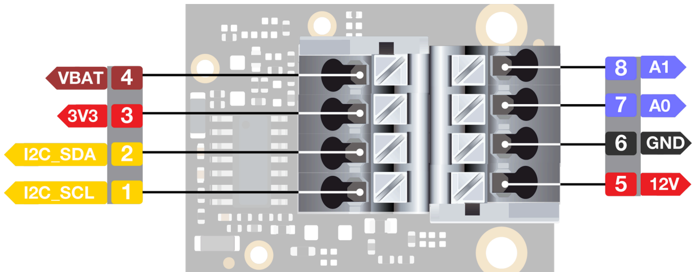
Figure 2: RAK5801 Sensor Connector
