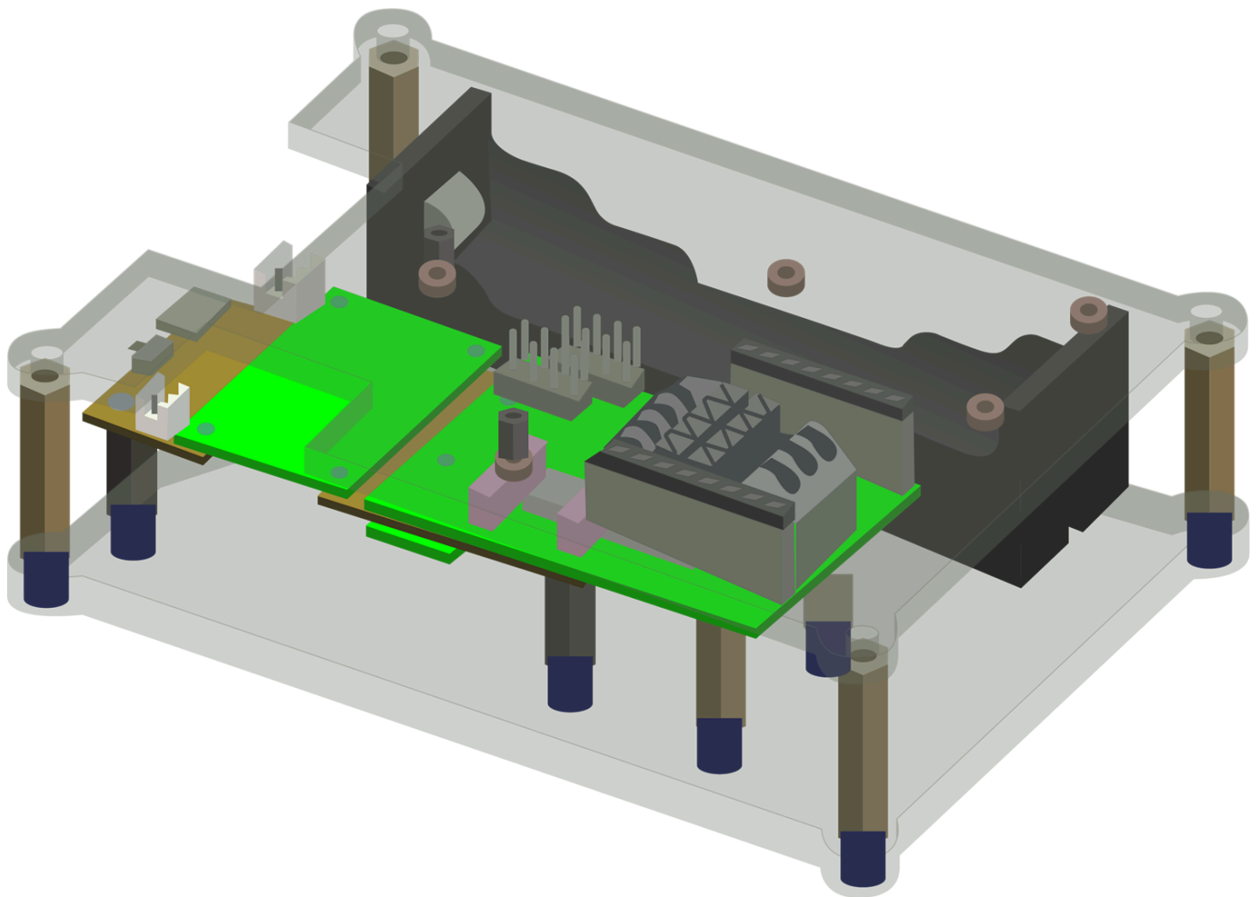
Figure 1: WisBlock RAKBox-B5 Enclosure Overview
