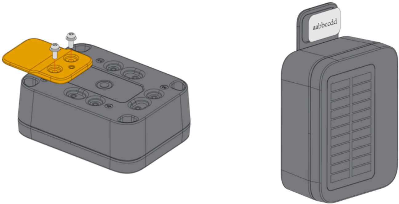
Figure 14: Label mount
