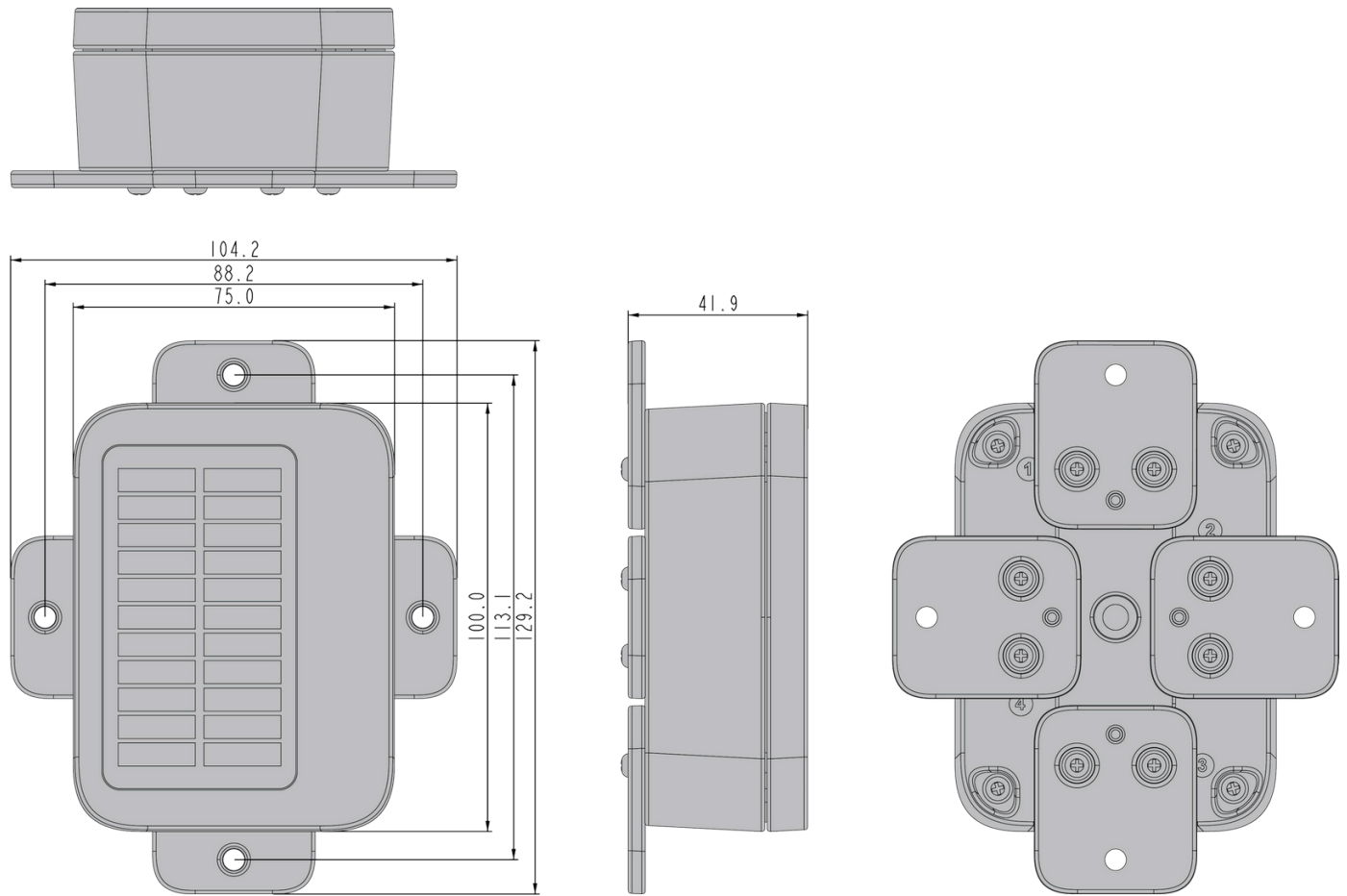
Figure 5: Dimensions of the enclosure with wall mount
