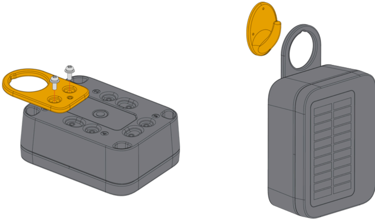
Figure 16: Hook loop mount
