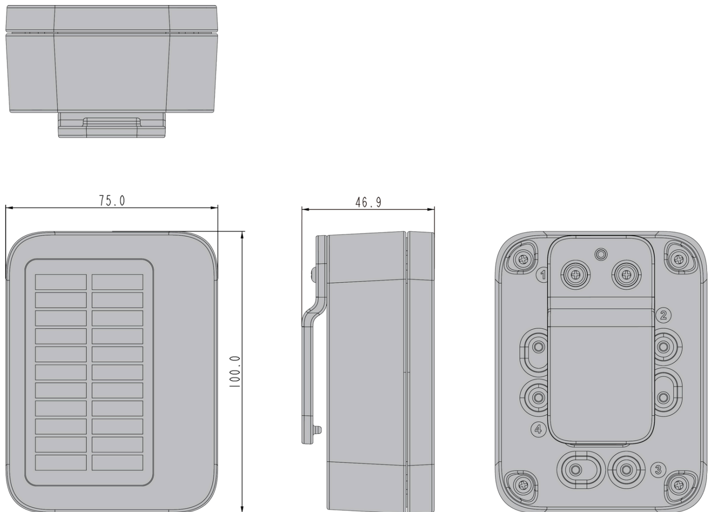
Figure 7: Dimensions of the enclosure with belt clip mount
