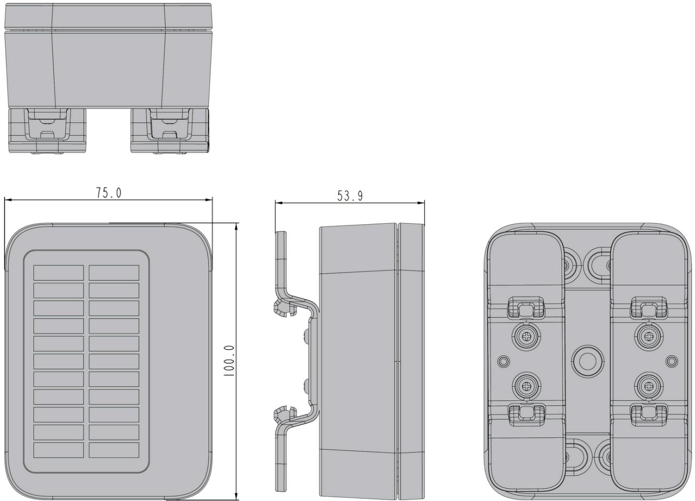
Figure 9: Dimensions of the enclosure with DIN mount
