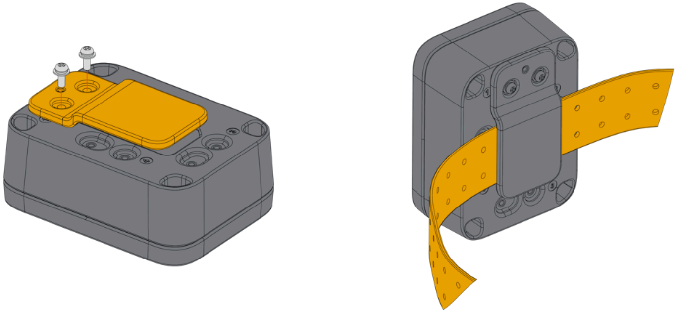
Figure 6: Belt clip mount
