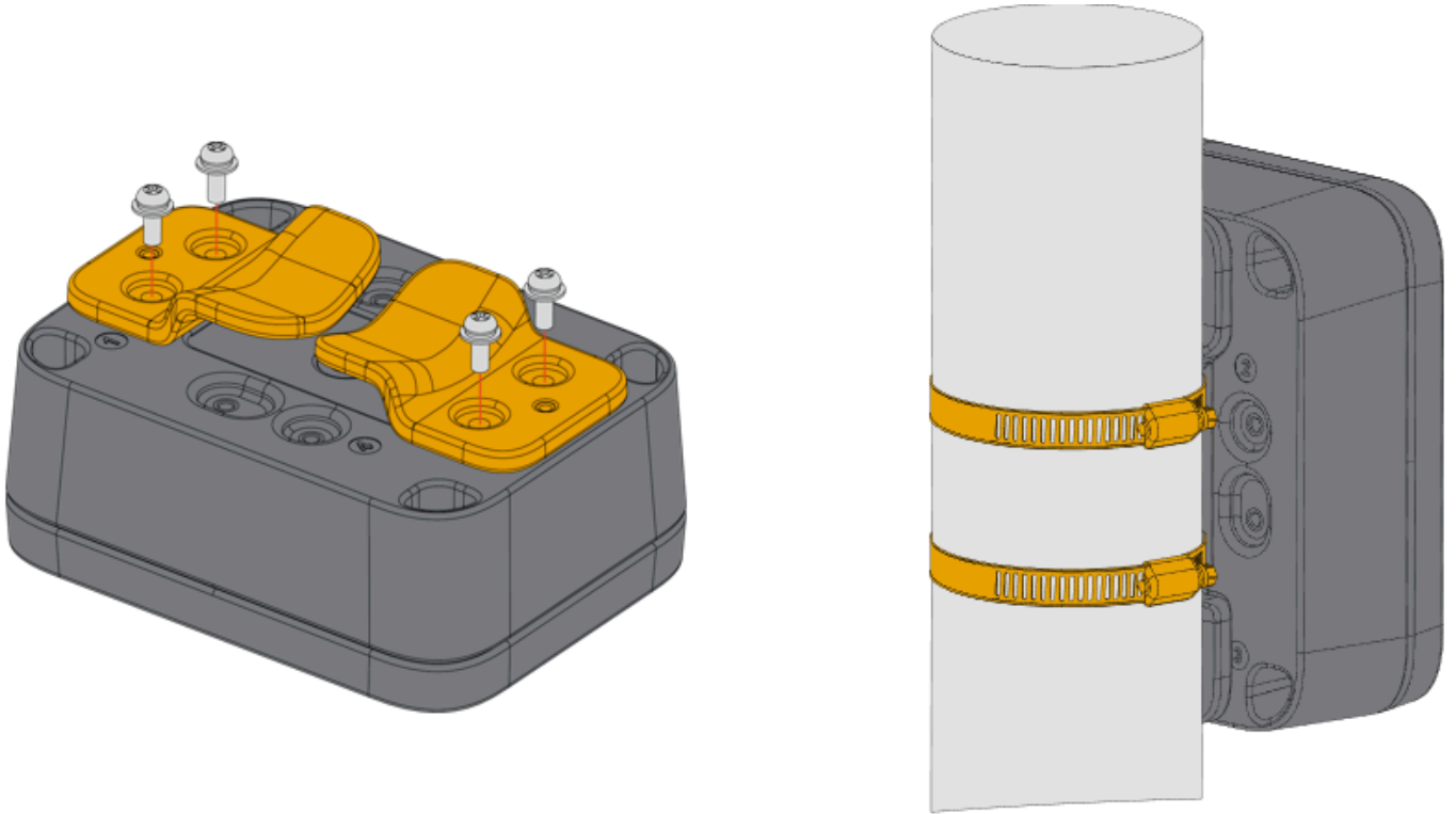
Figure 2: Vertical pole mount
