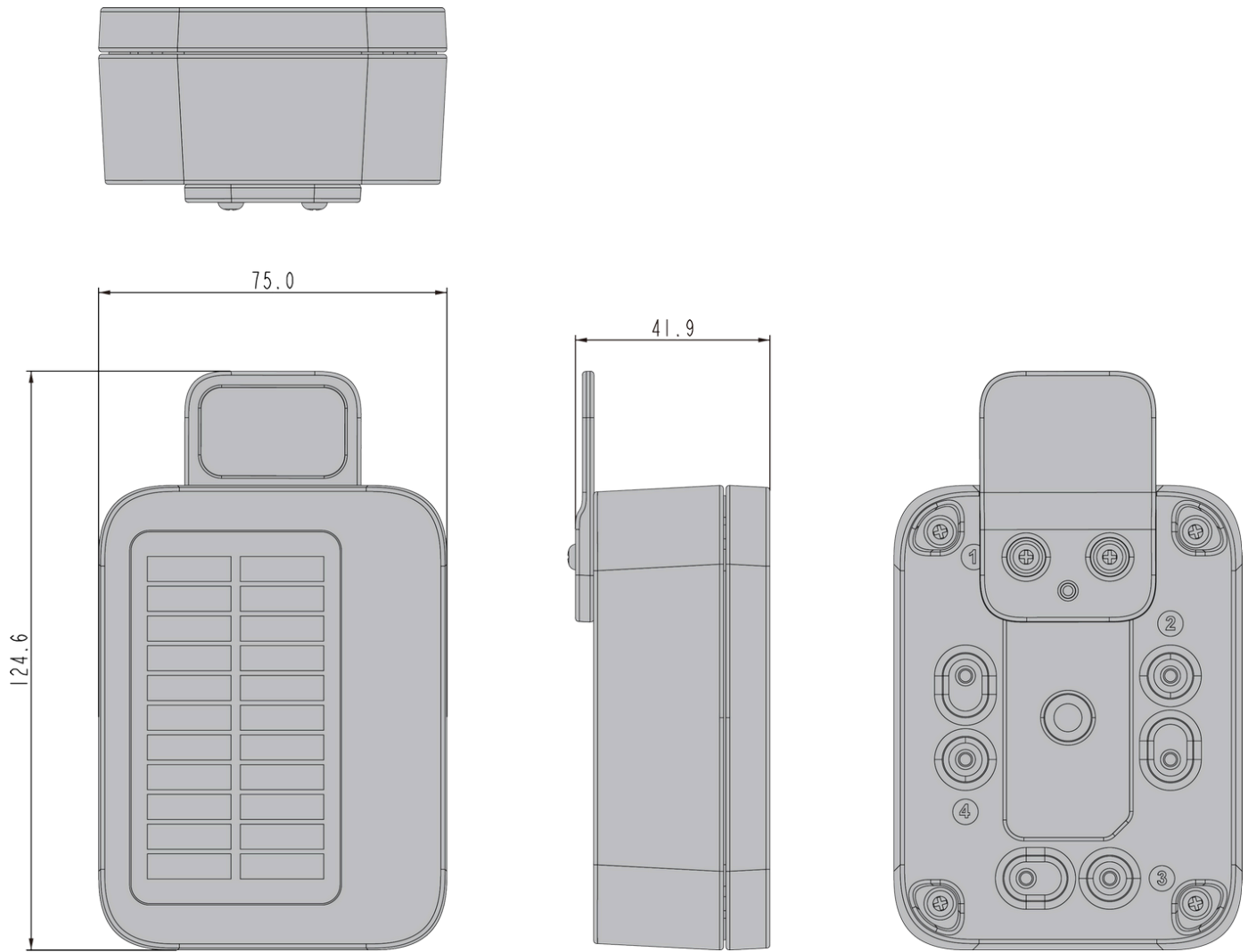
Figure 15: Dimensions of the enclosure with label mount
