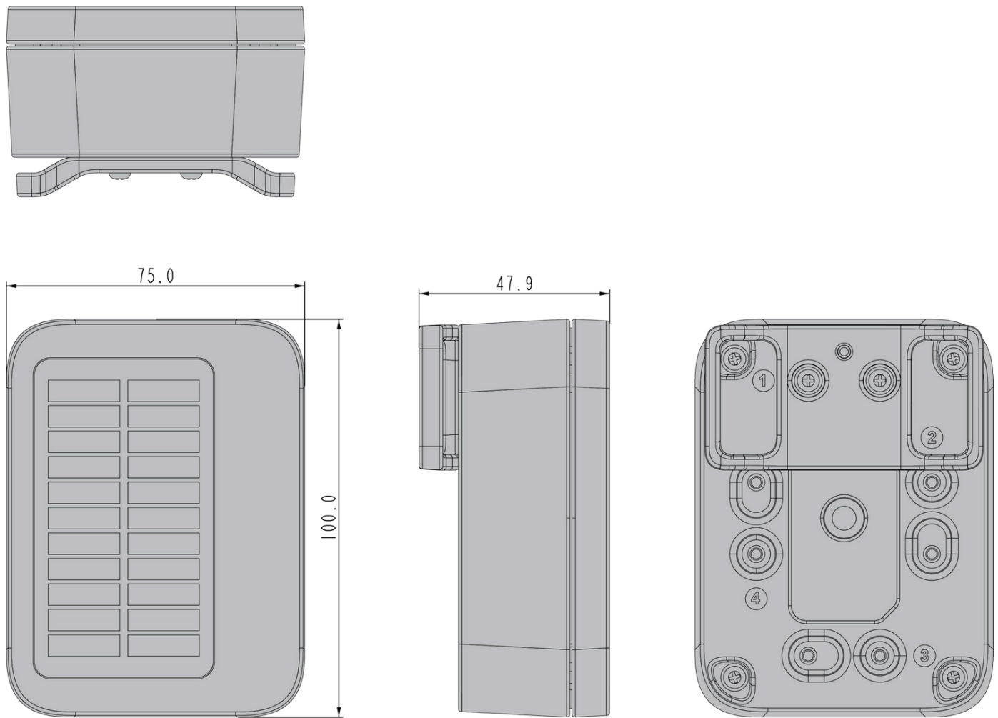
Figure 13: Dimensions of the enclosure with belt loop mount
