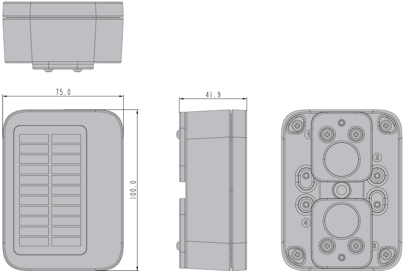
Figure 11: Dimensions of the enclosure with magnet mount
