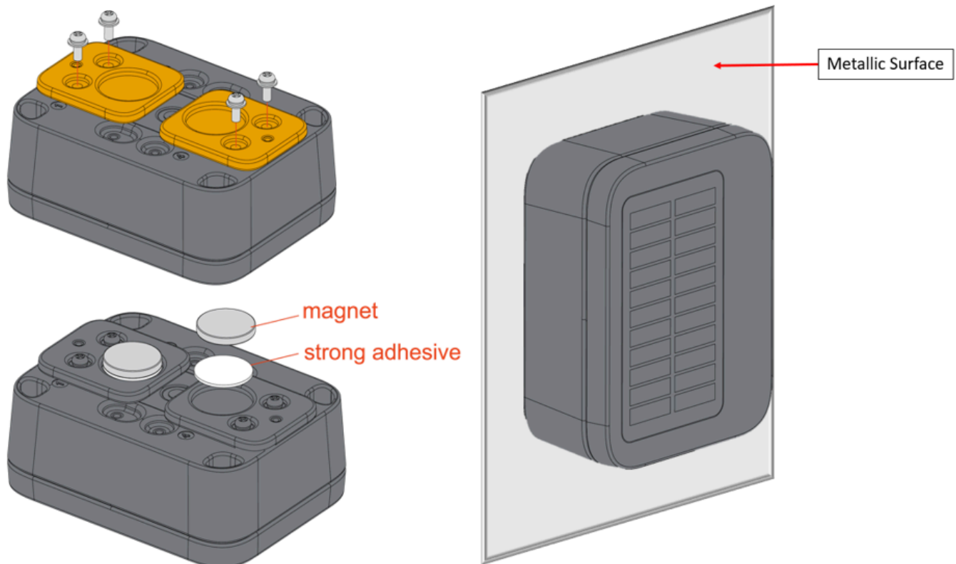
Figure 10: Magnet mount
