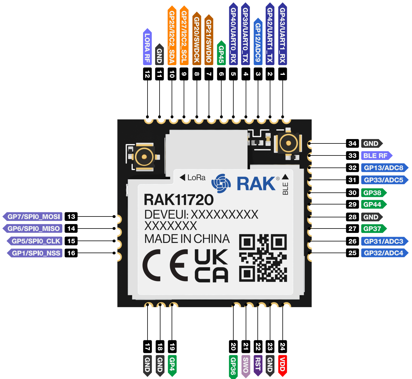
Figure 2: RAK11720 Pin Illustration
