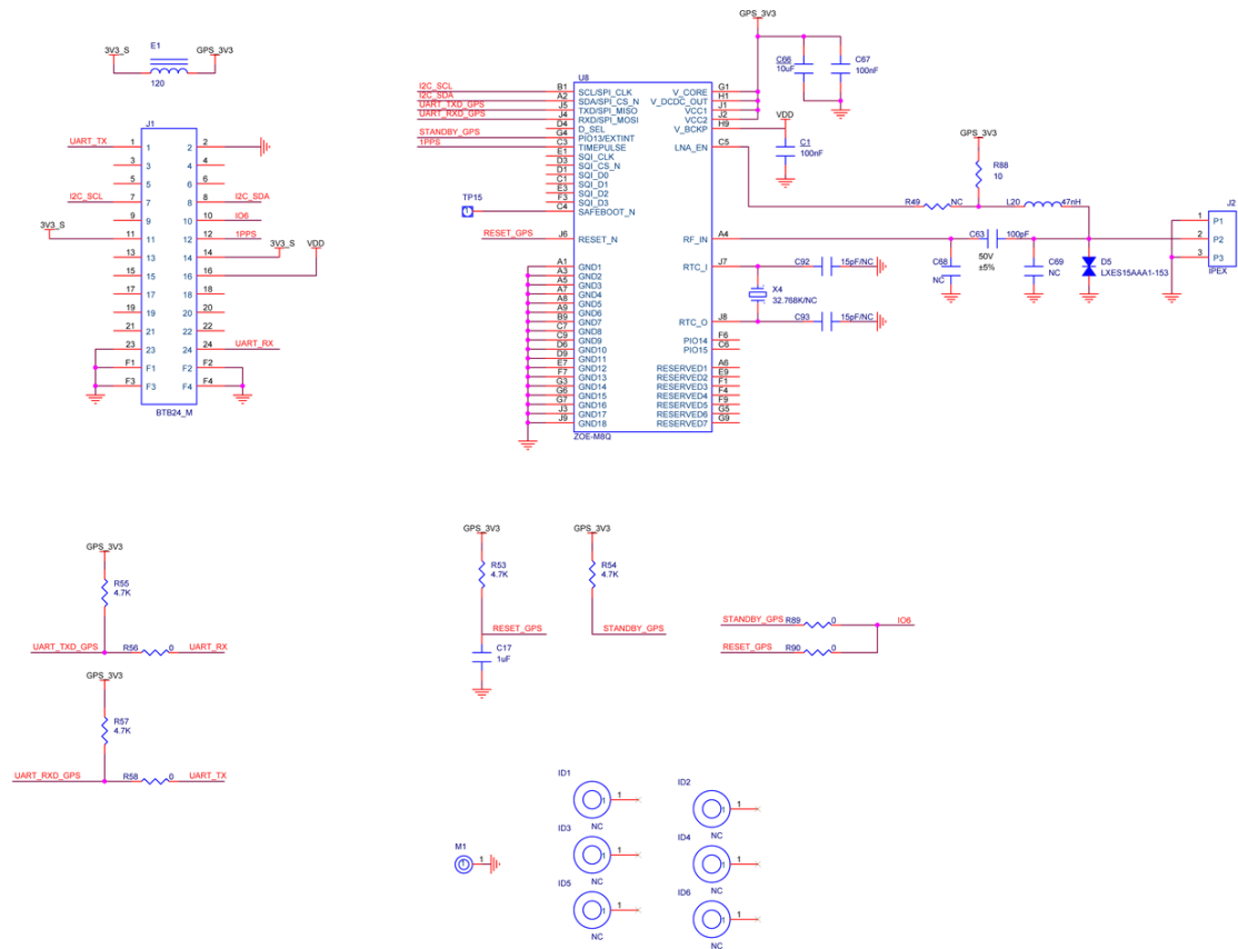
Figure 6: RAK12500 Schematic
