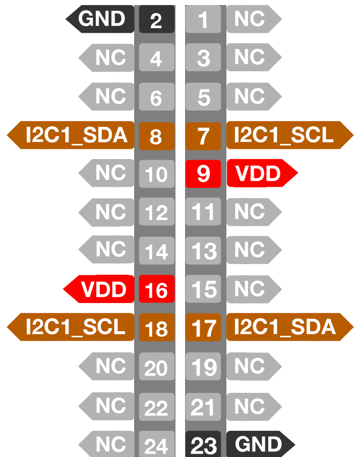
Figure 3: RAK1906 WisBlock Environmental Sensor Pinout
