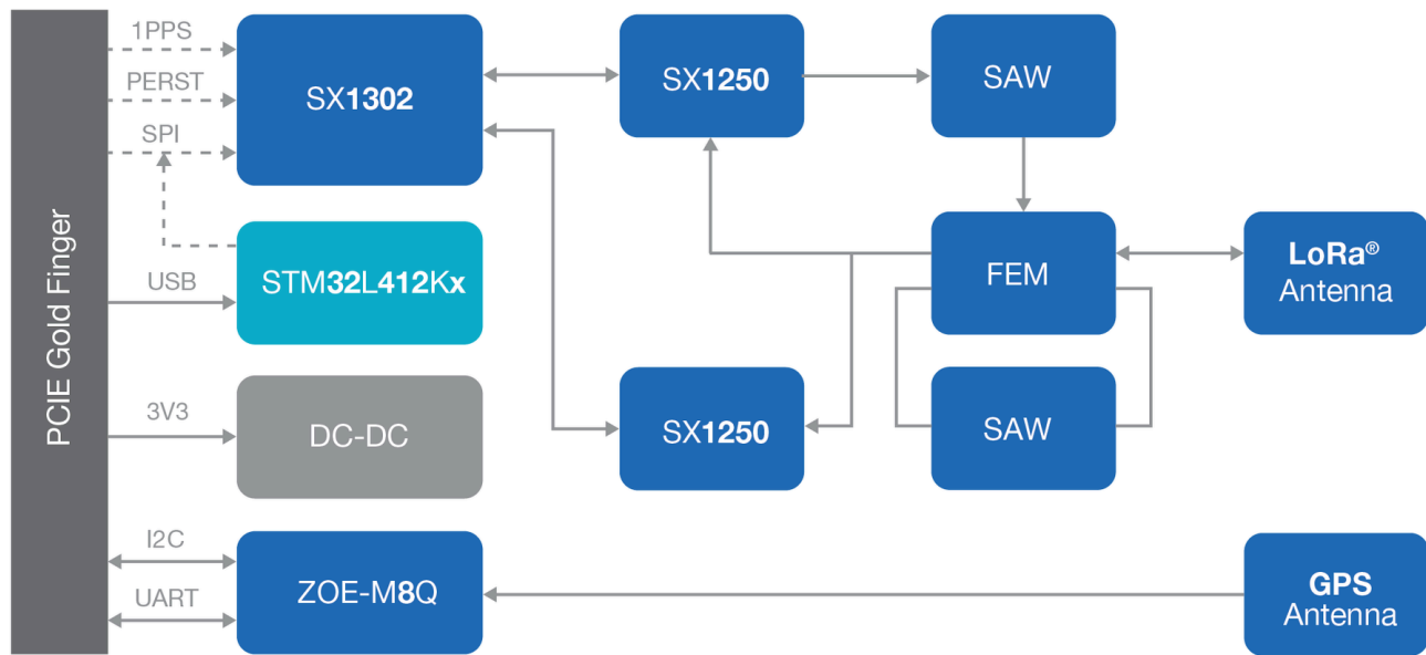
Figure 2: RAK2287 Block Diagram
