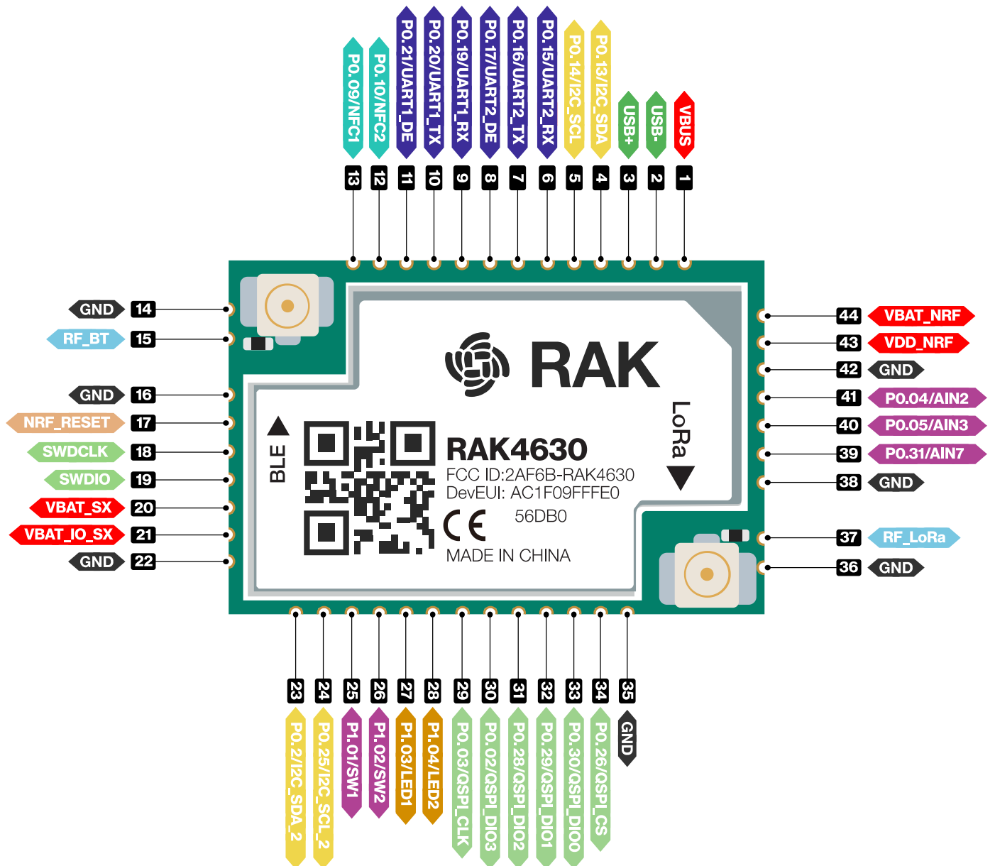
Figure 1: RAK4630 module pinout diagram
