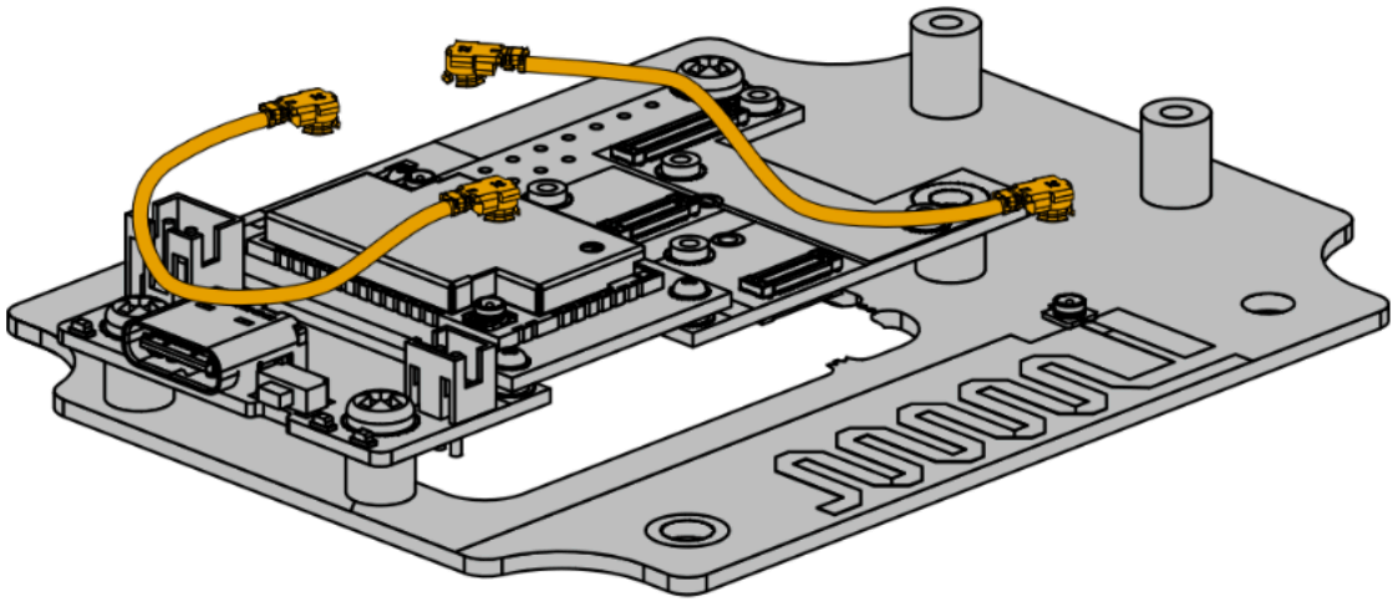
Figure 6: IPEX Connector of the Antenna
