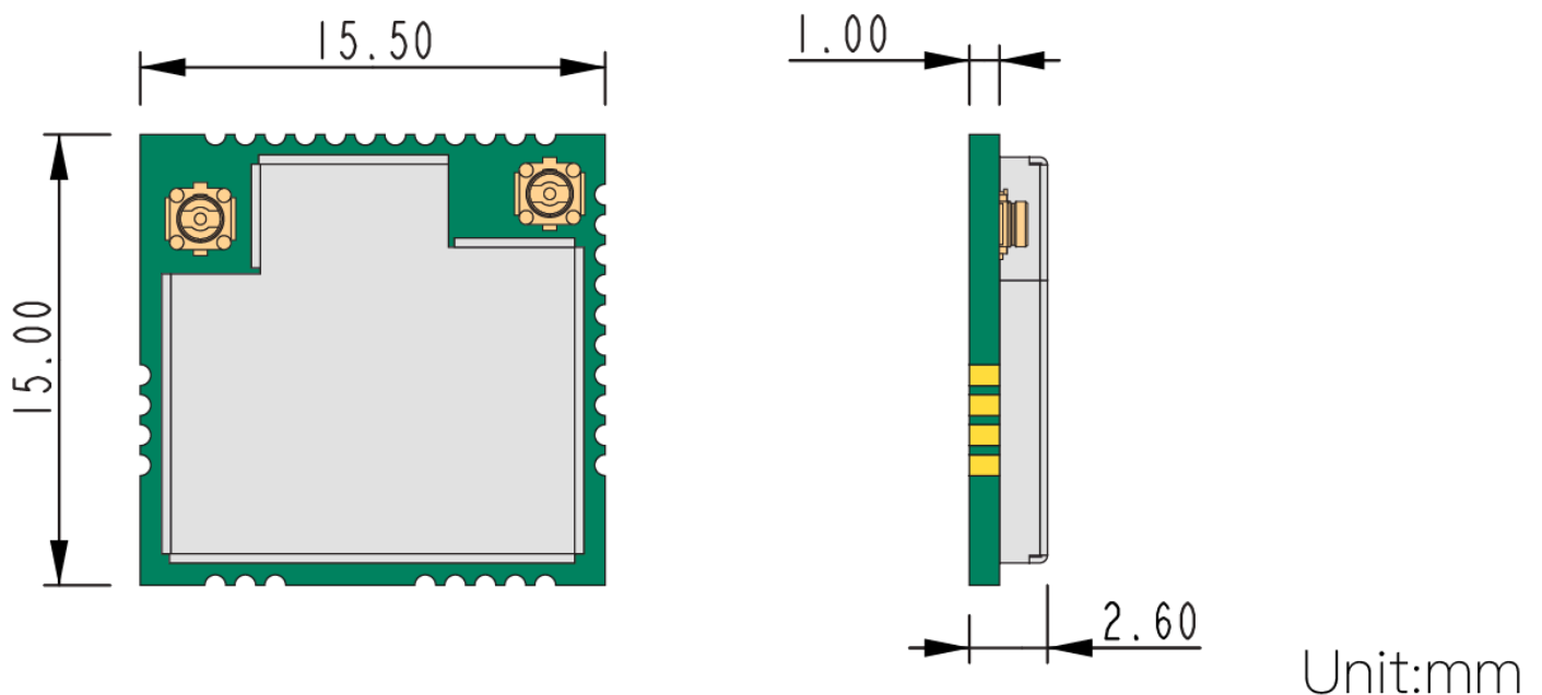
Figure 3: Board dimension
