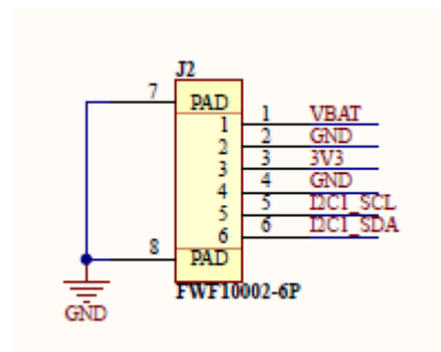
Figure 9: J2 Connector Pinout
