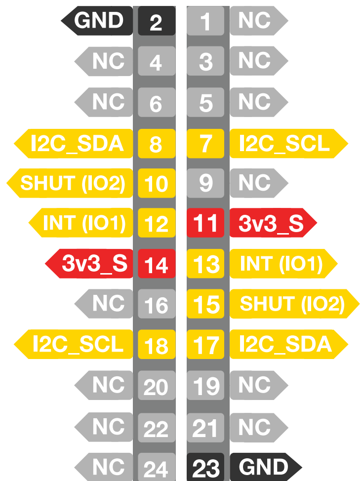
Figure 2: RAK12014 WisBlock ToF Sensor Module Pinout
