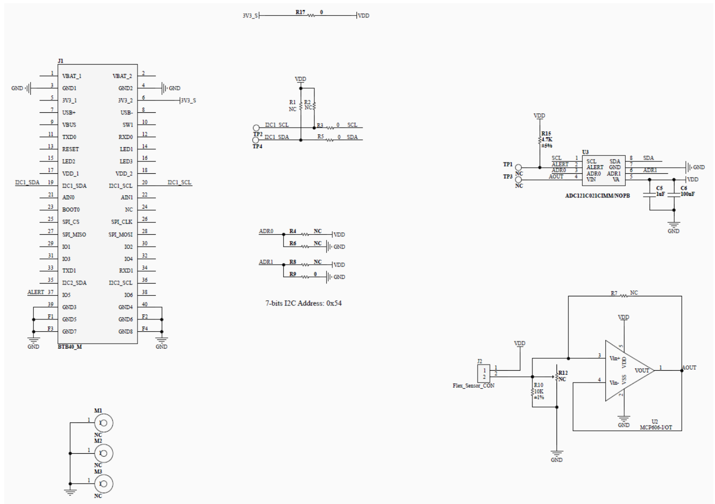
Figure 7: RAK12016 WisBlock Module Schematics
