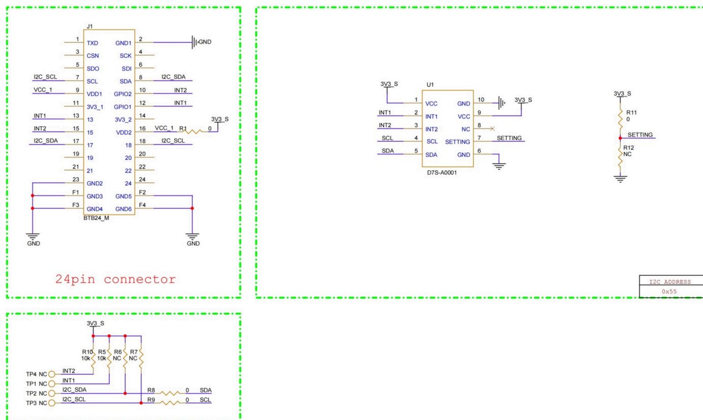
Figure 6: RAK12027 schematic diagram
