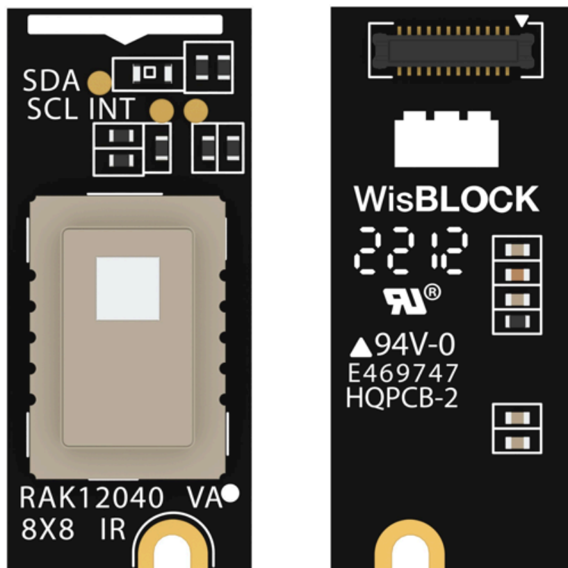
Figure 1: RAK12040 WisBlock 8x8 IR Sensor
