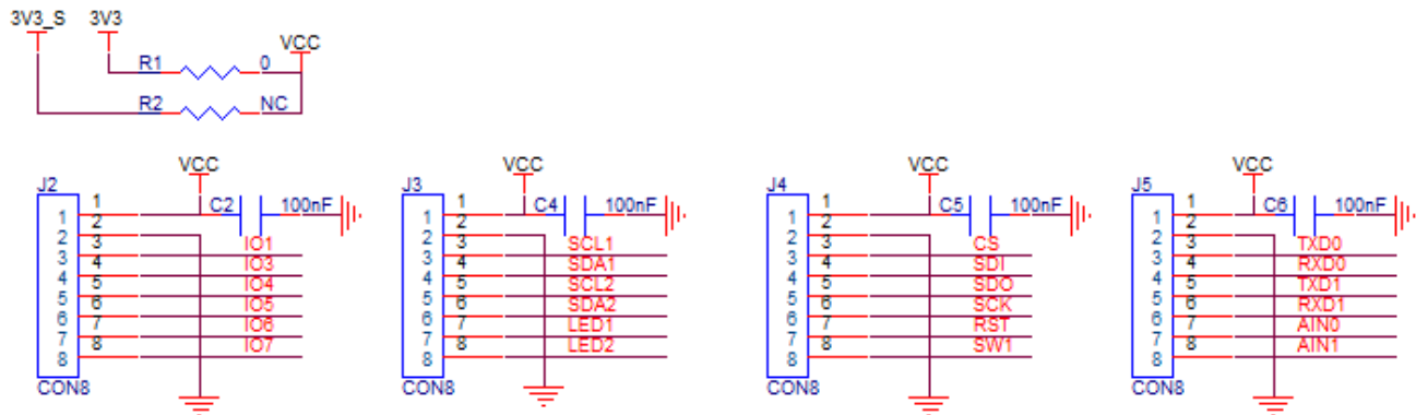
Figure 5: RAK13002 WisBlock Adaptor Schematic
