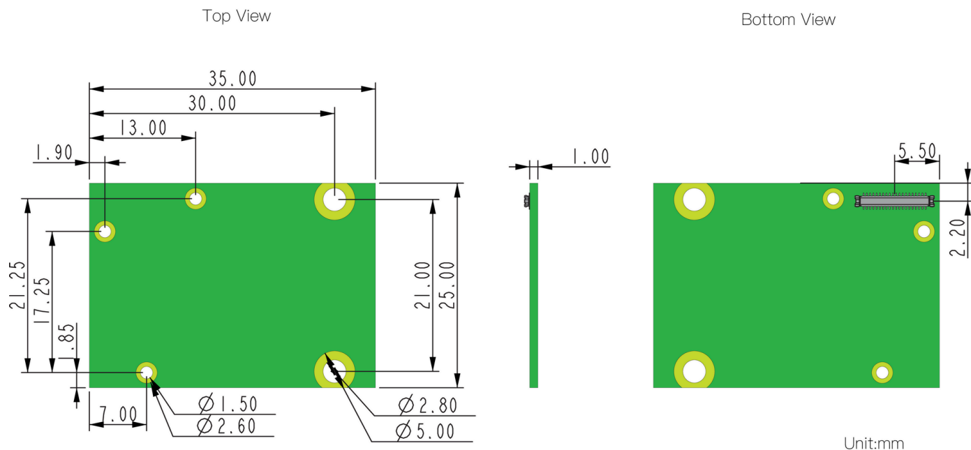
Figure 3: RAK13002 WisBlock Adaptor Module Mechanic Drawing
