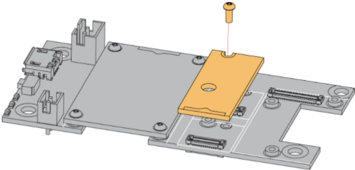
Figure 2: RAK13011 WisBlock Magnetic Switch Sensor Module Mounting
