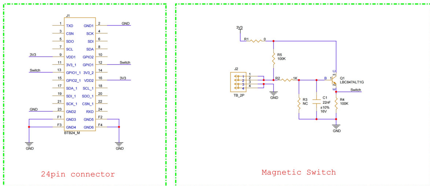
Figure 6: RAK13011 WisBlock Magnetic Switch Sensor Module Schematic
