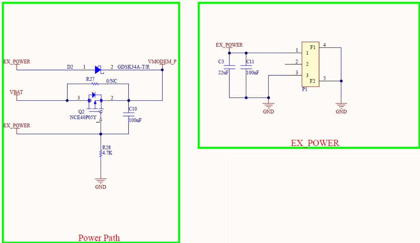
Figure 7: RAK13102 Power Supply
