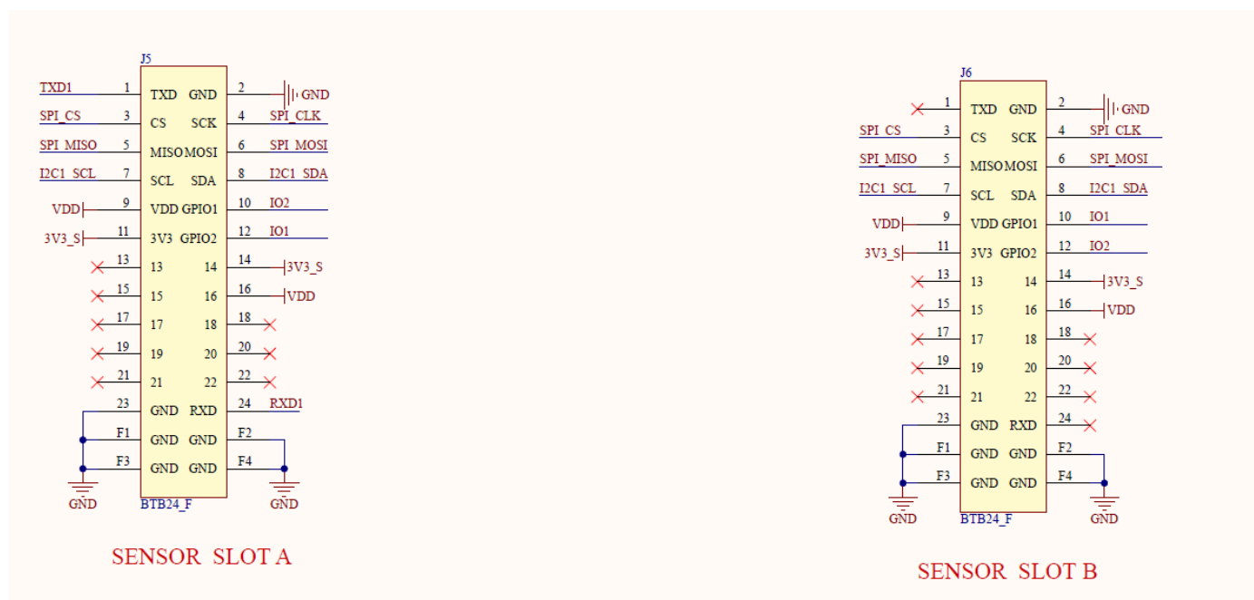
Figure 12: RAK13102 Module Sensor Slots
