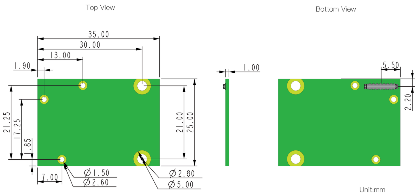
Figure 4: RAK14014 mechanical dimensions
