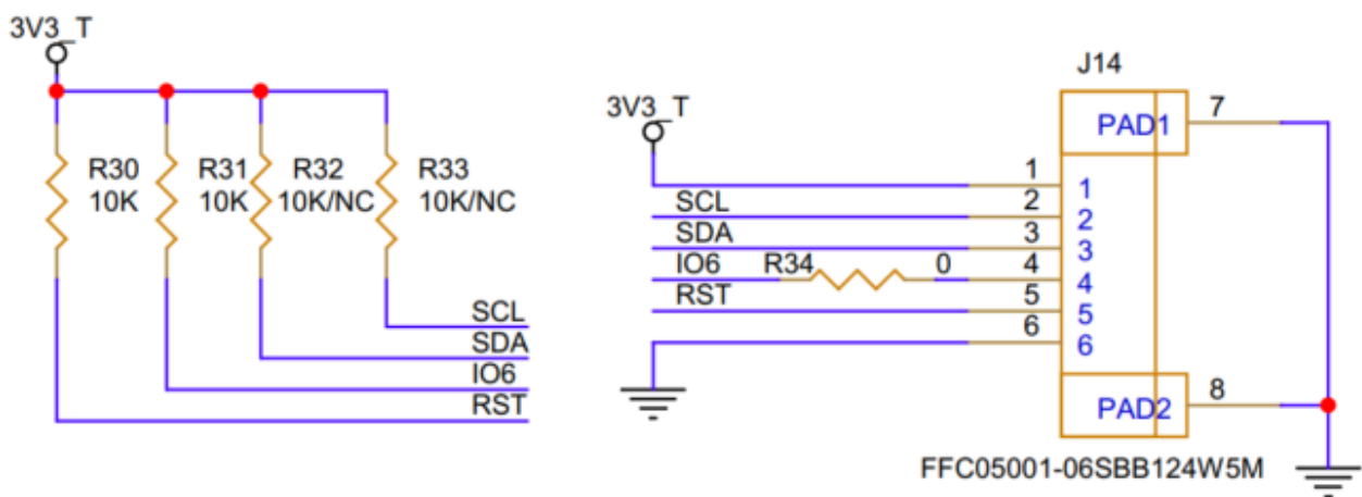
Figure 7: RAK14014 WisBlock Touch Drive Circuit
