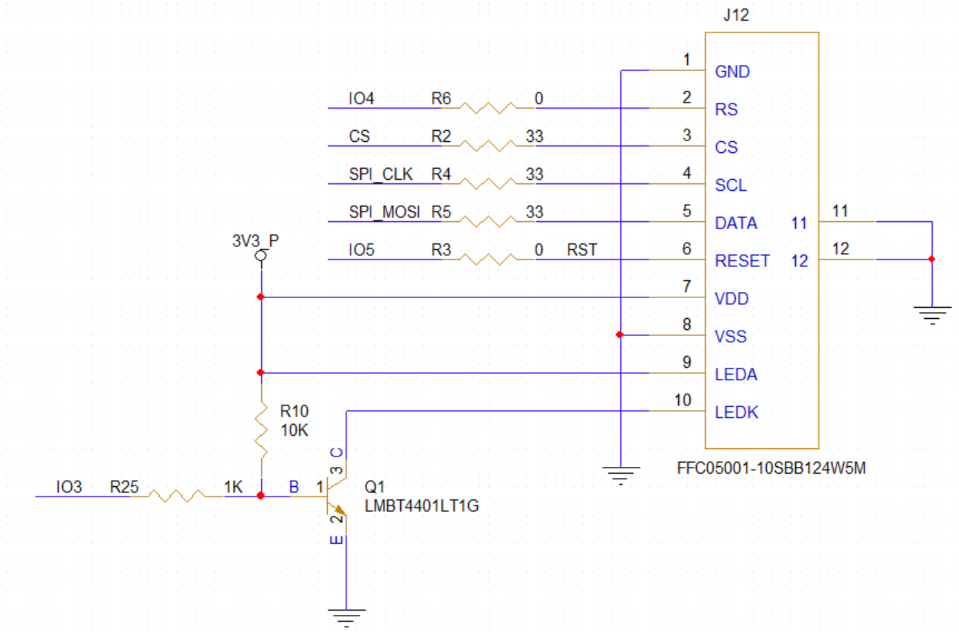
Figure 6: Display Connector Schematic diagram
