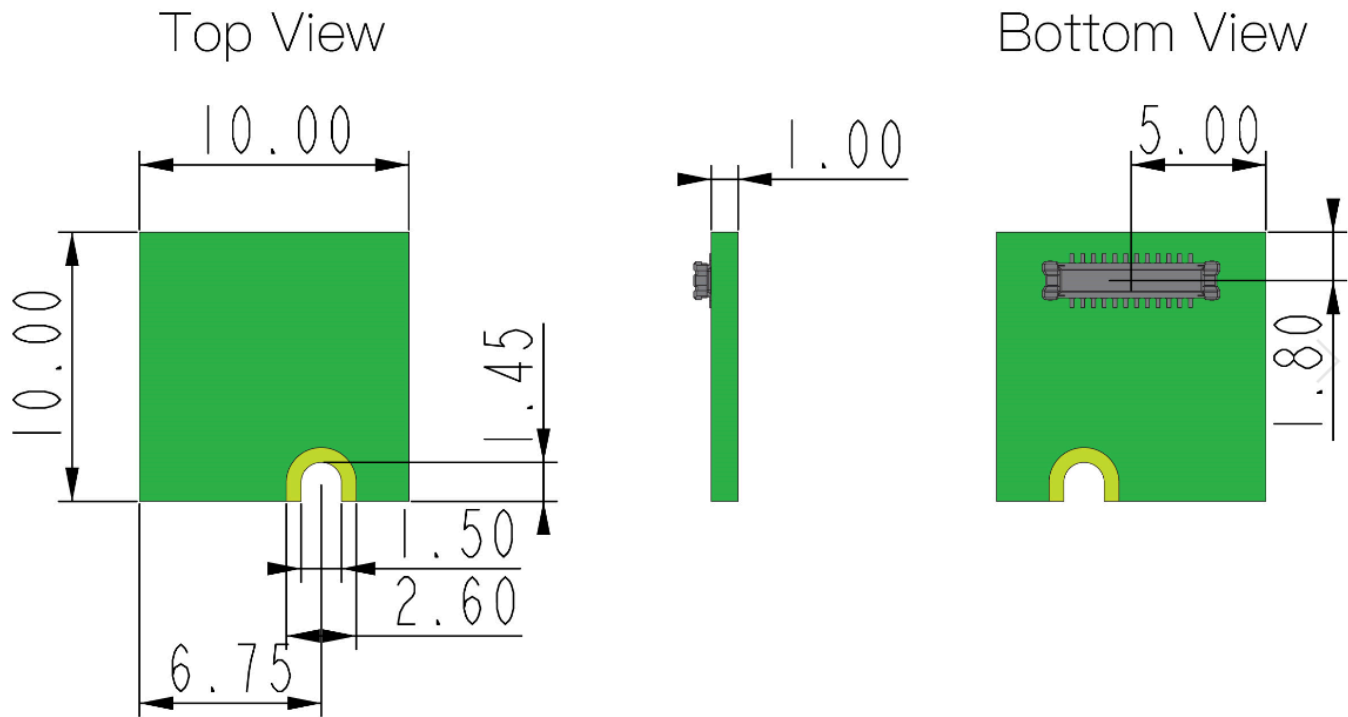
Figure 4: RAK15003 WisBlock 32kByte FRAM Module Mechanic Drawing
