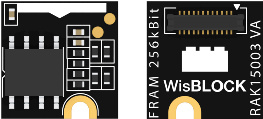
Figure 1: RAK15003 WisBlock 32kByte FRAM Module
