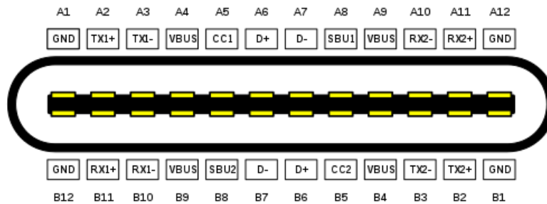
Figure 4: USB Type-C receptacle pinout
