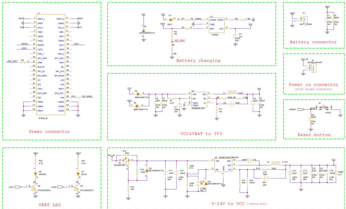
Figure 8: RAK19016 5~24 V Power Slot Module schematics
